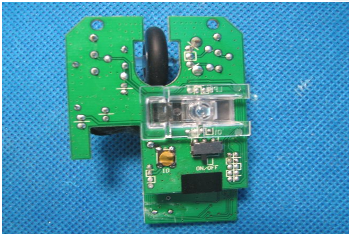
Fig.7- Interview of SPM5801bottom PCB
