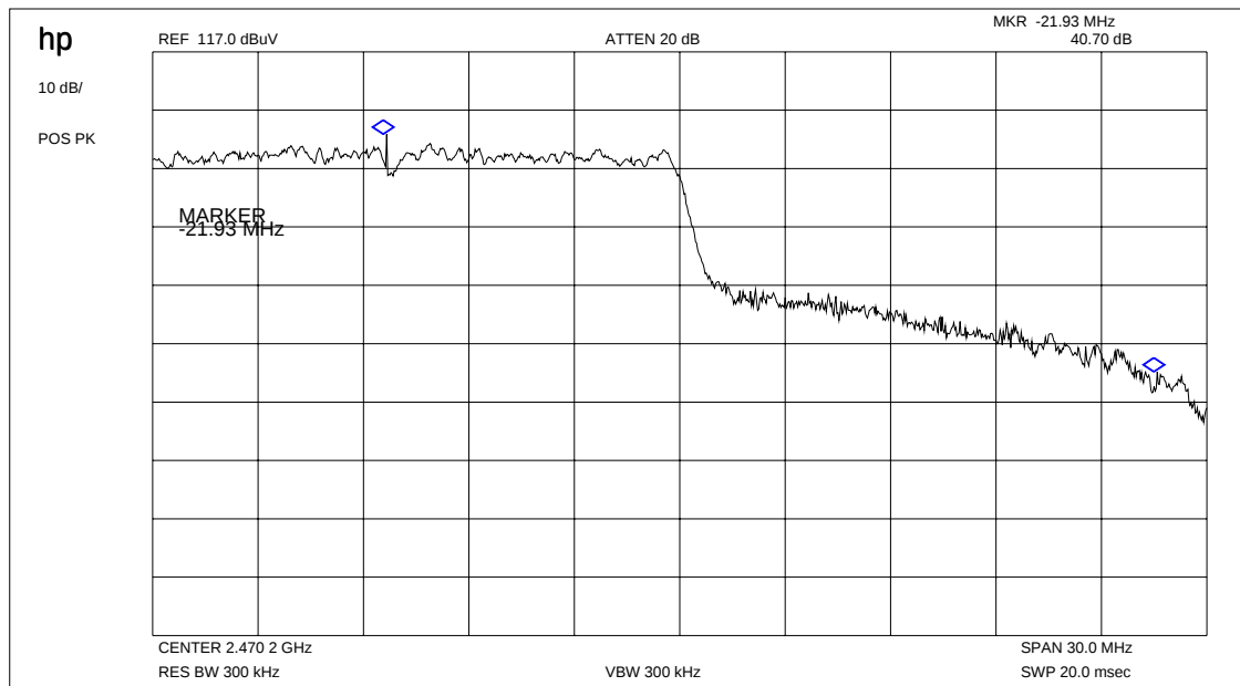
Plot 3: Marker-Delta Method RBW/VBW = 1% of span
