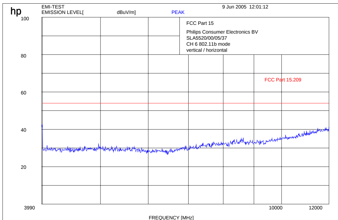
Plot 5: 4- 12 GHz (middle channel)
