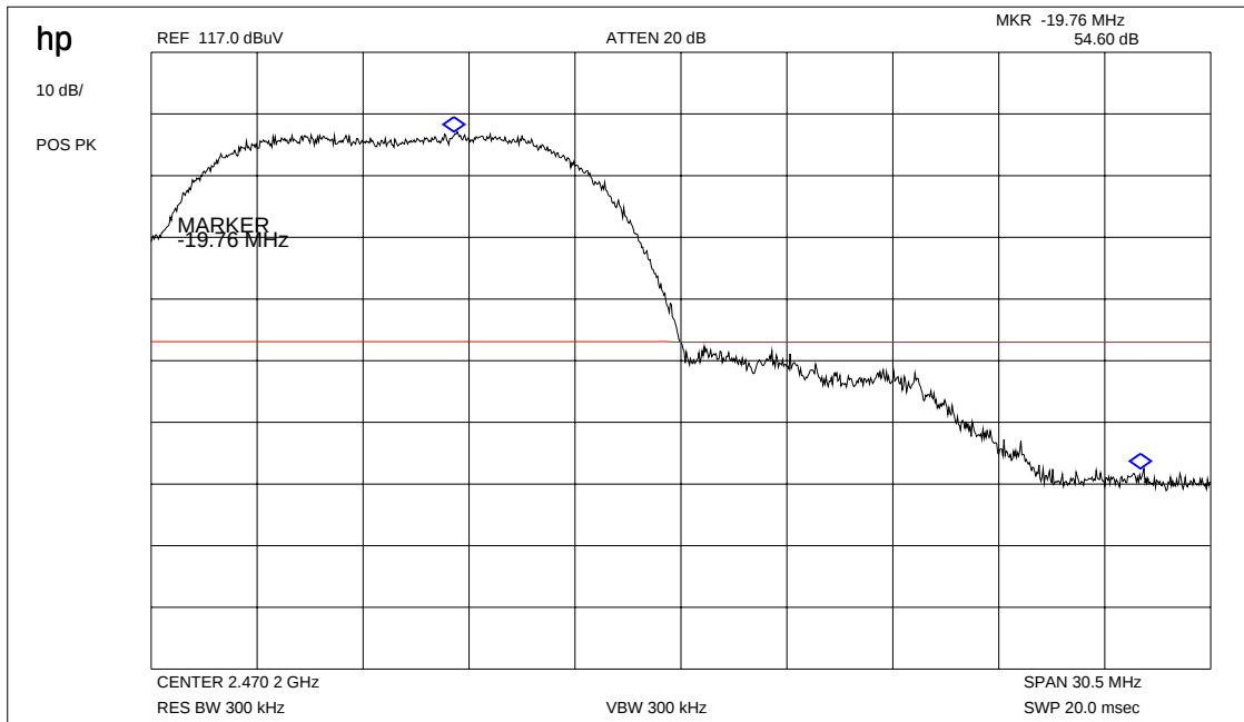
Plot 3: Marker-Delta Method RBW/VBW = 1% of span
