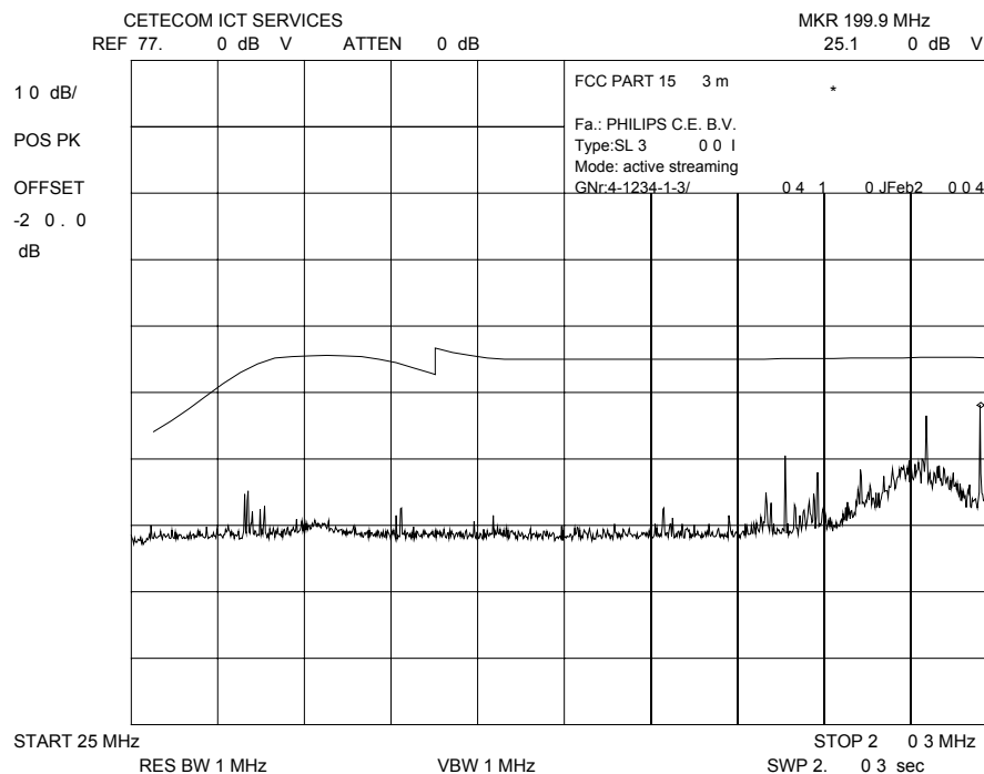
Plot 9: 0.03 – 0.2 GHz horizontal (middle channel)
