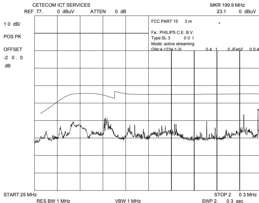
Plot 15: 0.03 – 0.2 GHz horizontal (highest channel)
