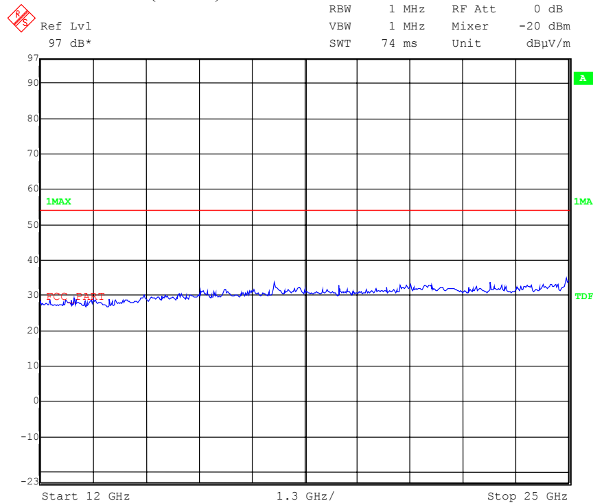
Plot 3: 12- 25 GHz horizontal / vertical (receiver)
