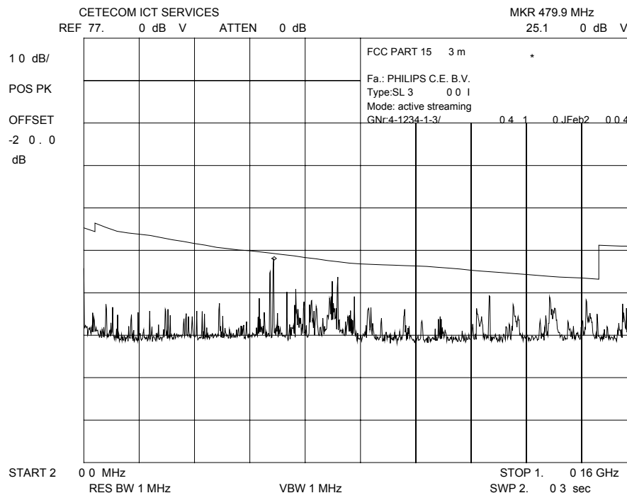
Plot 11: 0.2 – 1 GHz horizontal (middle channel)
