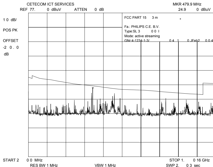
Plot 17: 0.2 – 1 GHz horizontal (highest channel)
