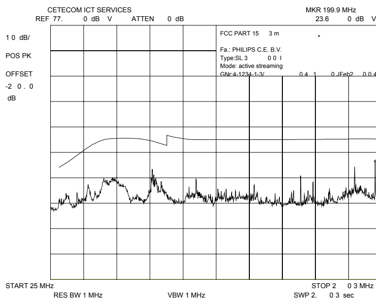
Plot 2: 0.03 – 0.2 GHz horizontal (lowest channel)
