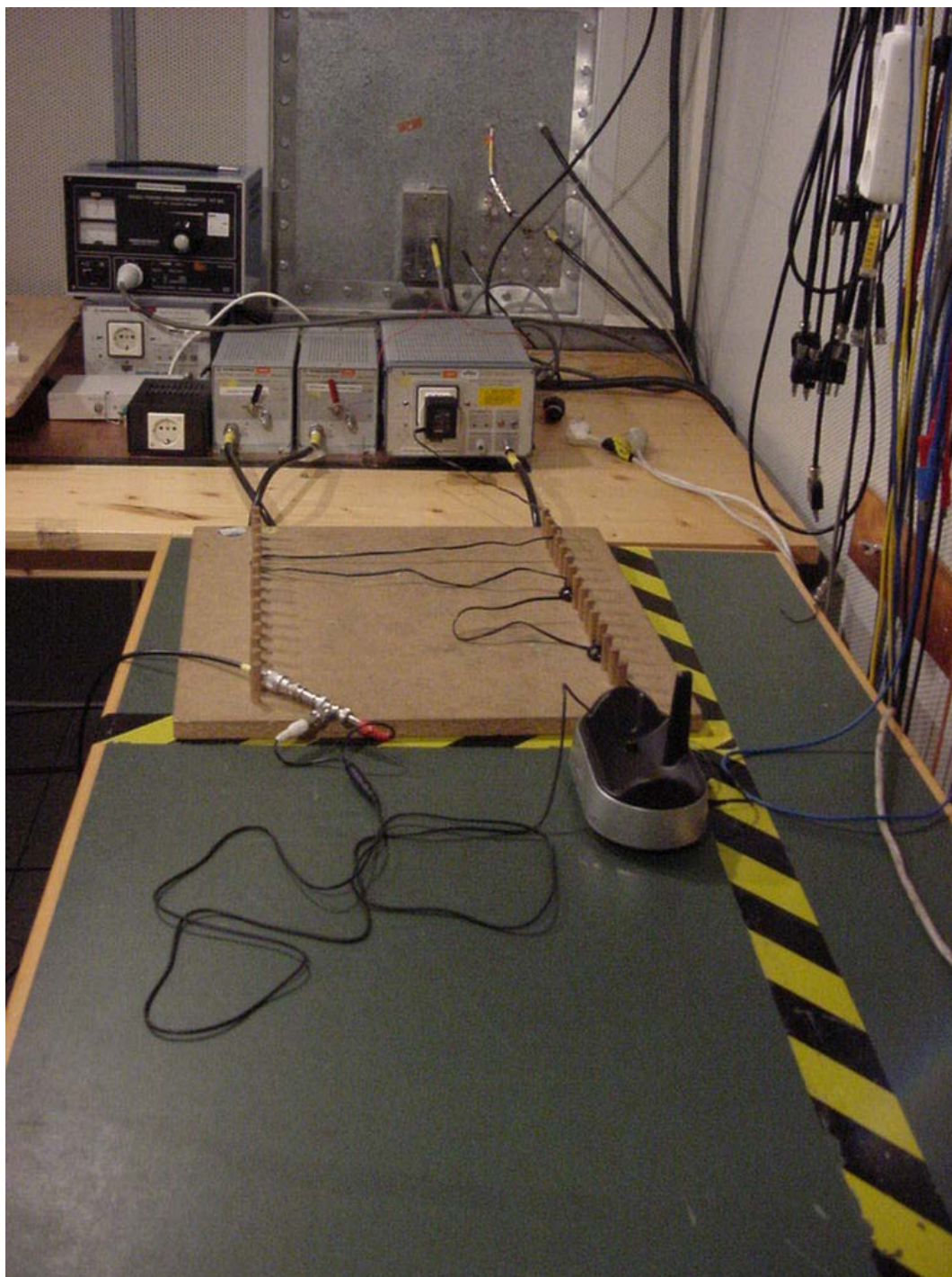
Photo 5 (Conducted Emissions): Tx mode
