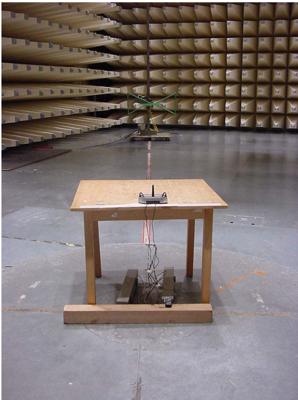
Photo 1 (Radiated Emissions): Tx Test set-up
