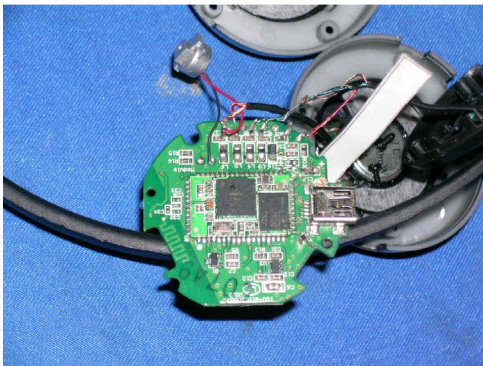
Headset Main PCB solder side
