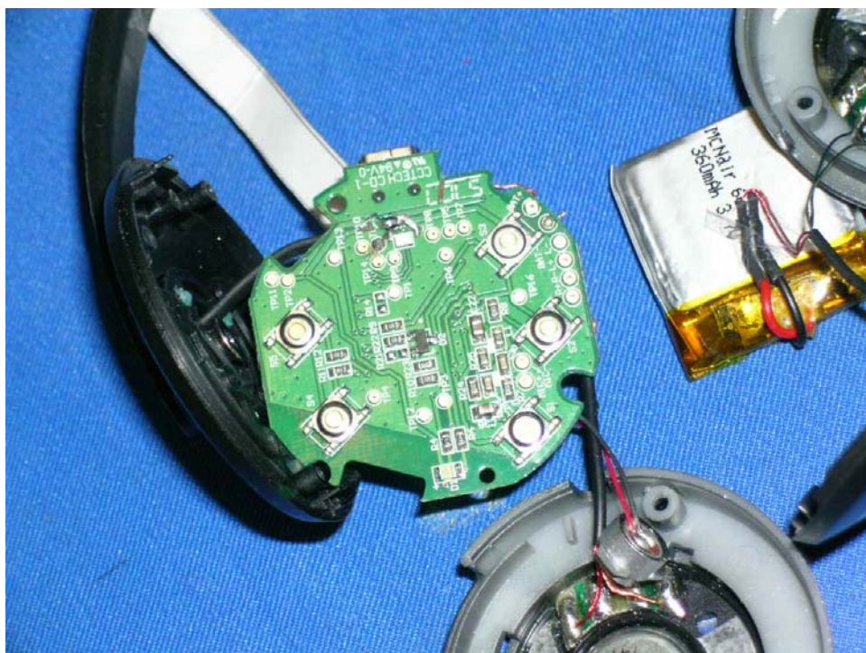
Headset Main PCB comp side
