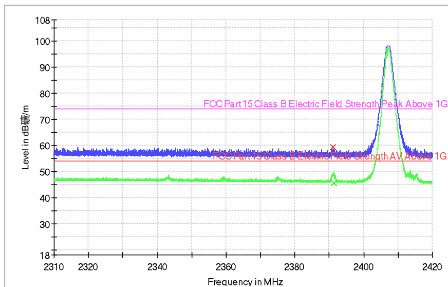
Electric Field Strength 1-18GdBuV TX
