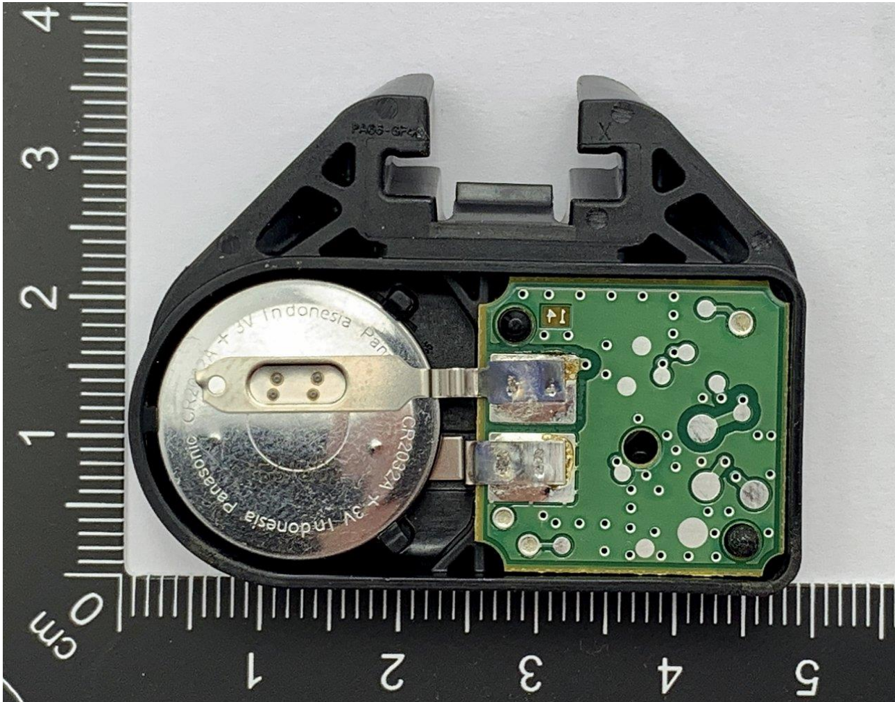
PCB & battery mounted in housing
