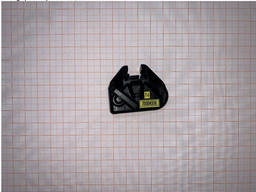
Photograph 6: Bottom side view, EUT C
