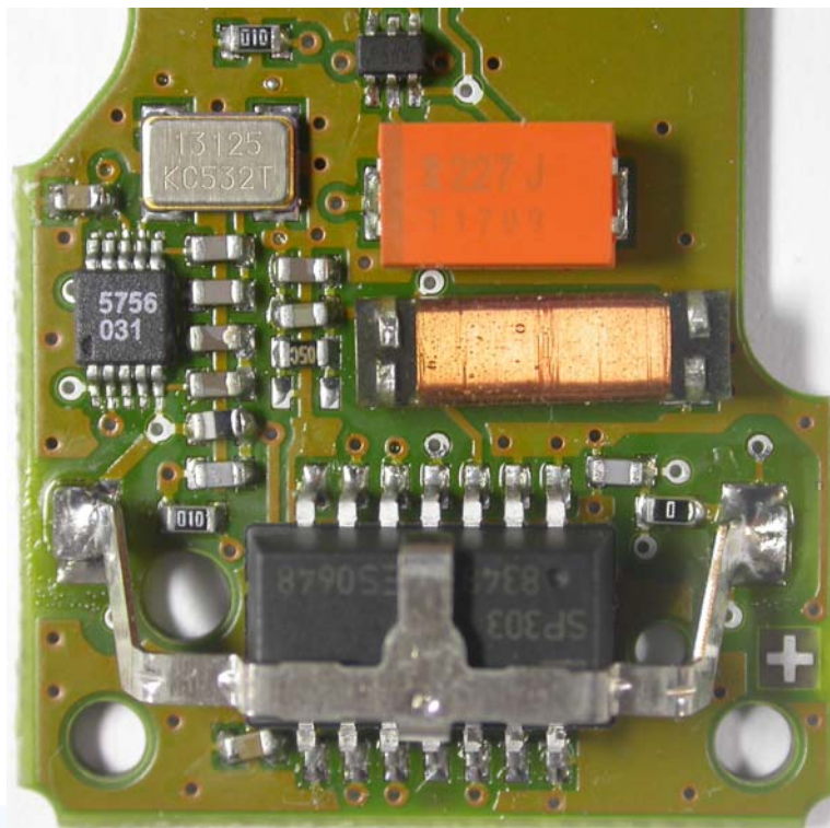
Wheel Electronic / TSSRE3Tc Internal Photo Part view of PCB
