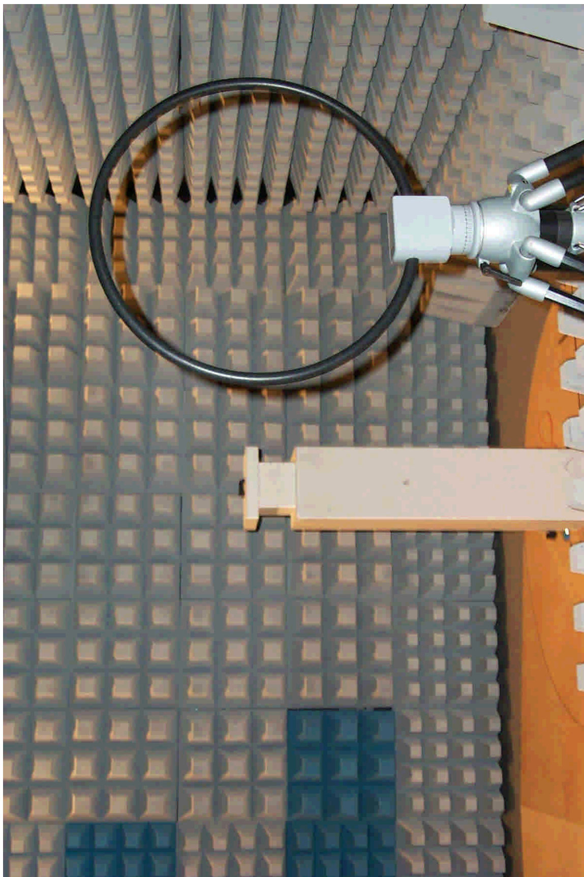
40458emi8.jpg: Test set-up preliminary radiated emission measurement 9 kHz to 30 MHz
