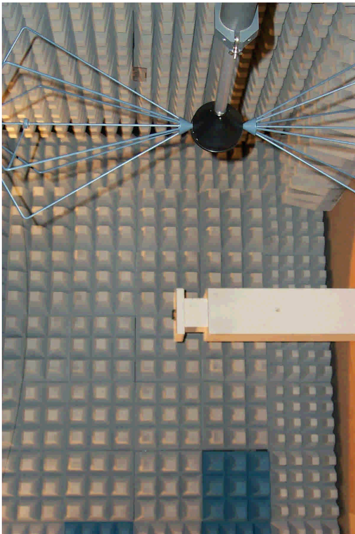
40458emi17.jpg: Test set-up radiated emission measurement 30 MHz to 1 GHz.
