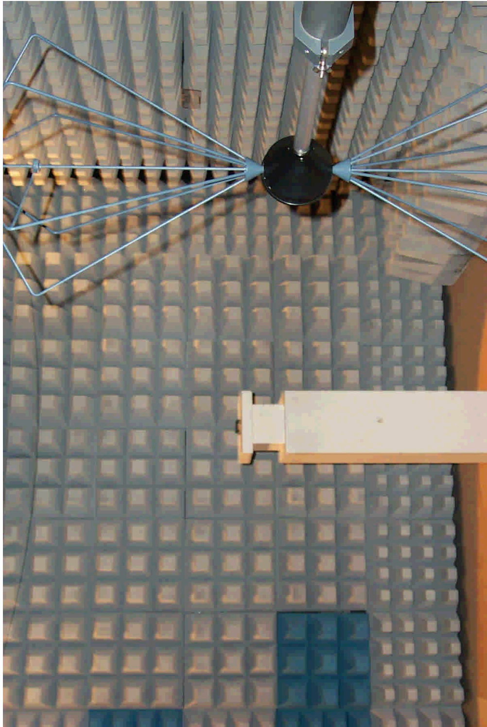
40448emi2.jpg: Test set-up preliminary radiated emission measurement
