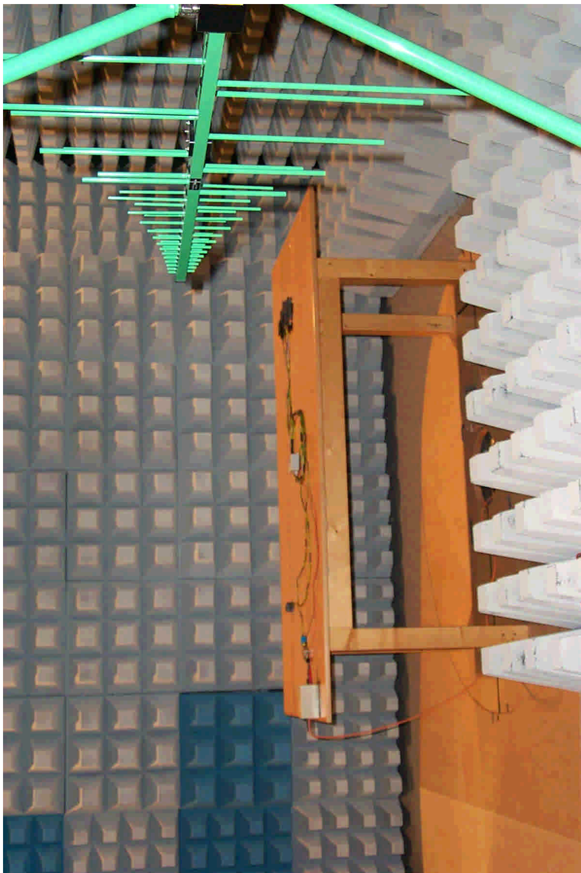
40458emi1.jpg: Test set-up preliminary radiated emission measurement 30 MHz to 1 GHz
