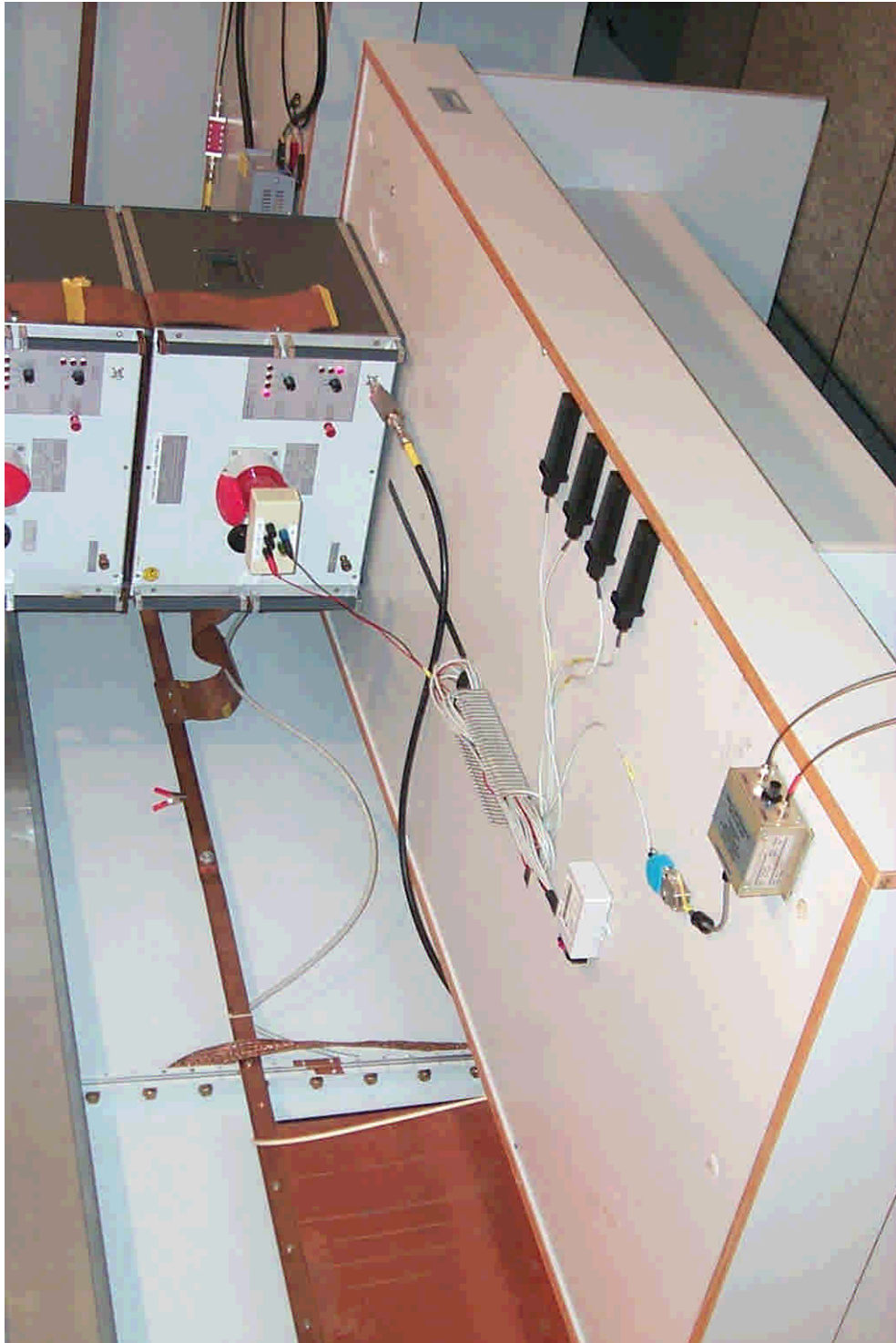
30759emi21.jpg Test set-up conducted emission
