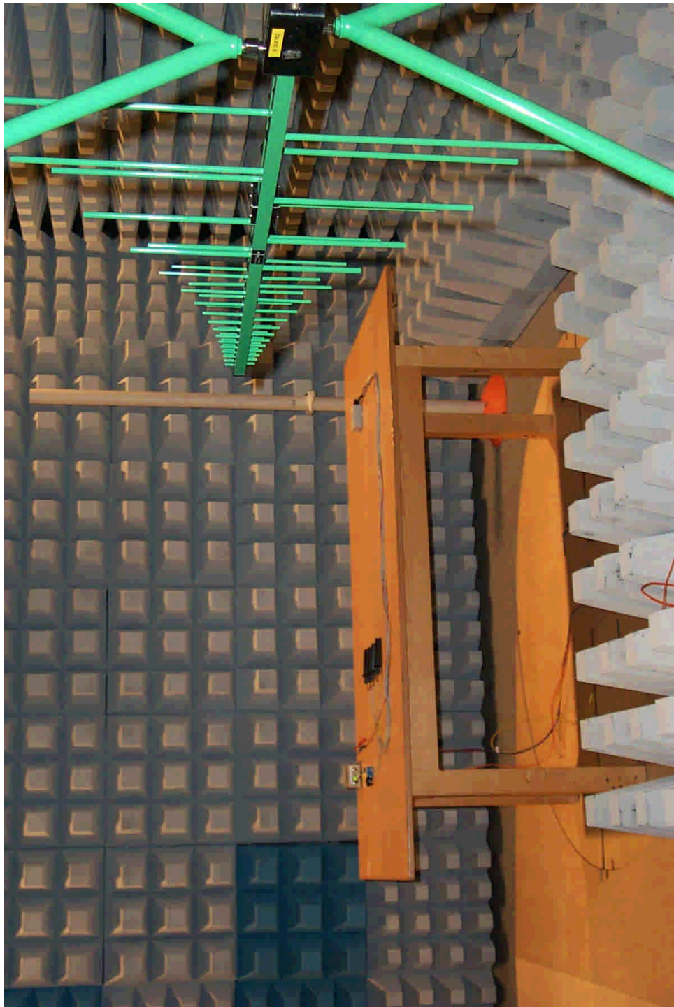
30759emi2.jpg Test set-up radiated emission (anechoic chamber)
