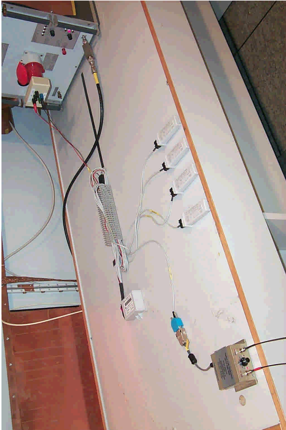
30759kfz3.jpg Test set-up conducted emission
