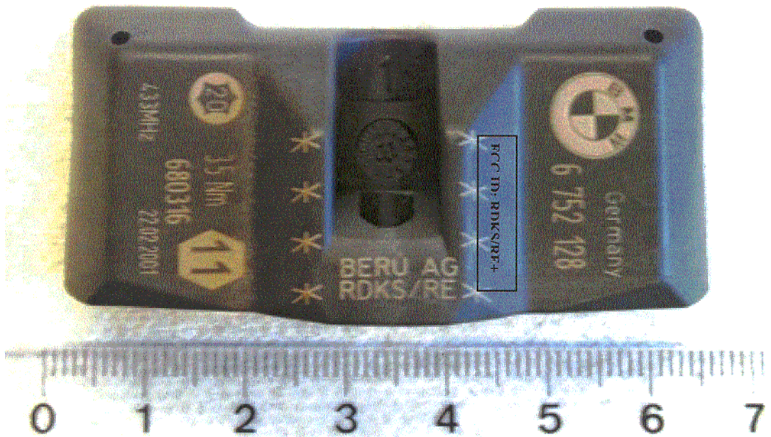
picture 1: top view of the transmitter RDKS / RE+ (magnification 2:1) remark: The FCC identifier will be located in the marked area. The rest of the labelling may vary.
