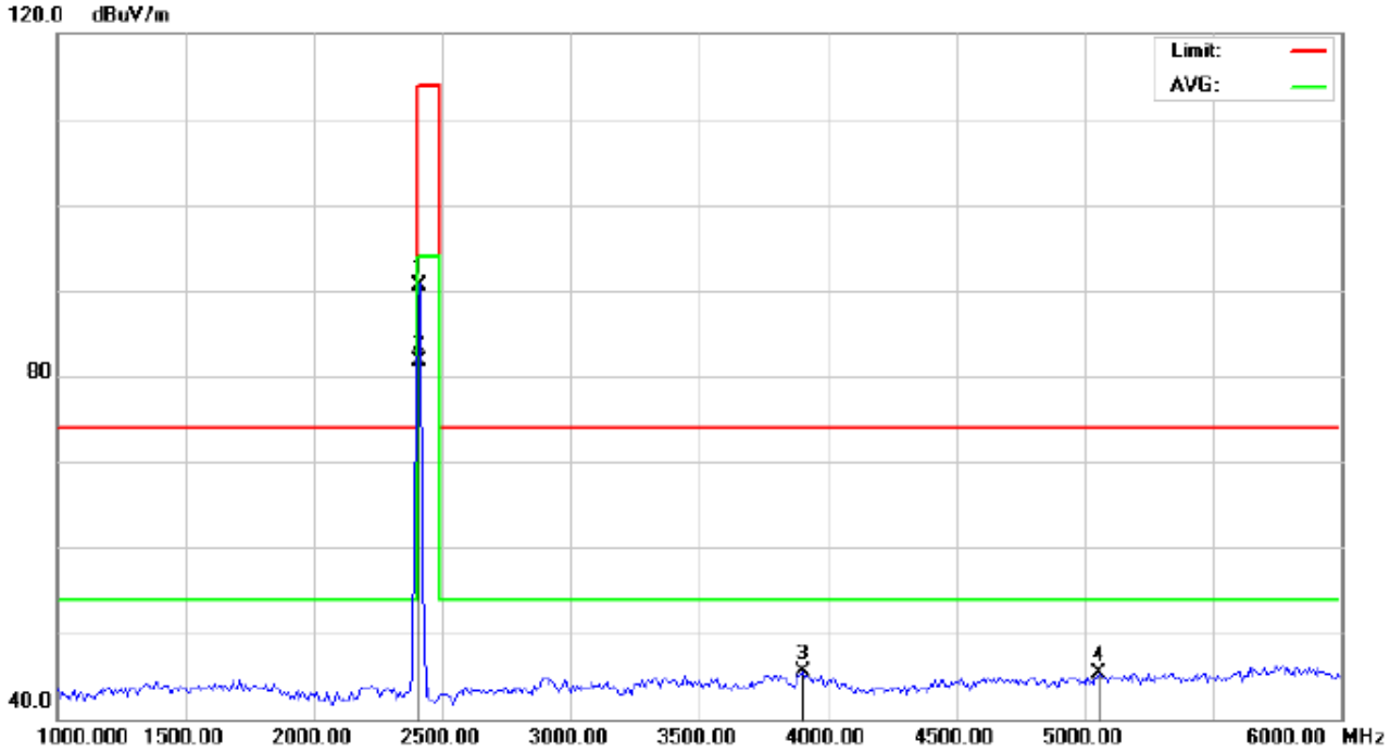
RADIATED EMISSION TEST- (ABOVE 1GHZ)-LOW CHANNEL-HORIZONTAL
