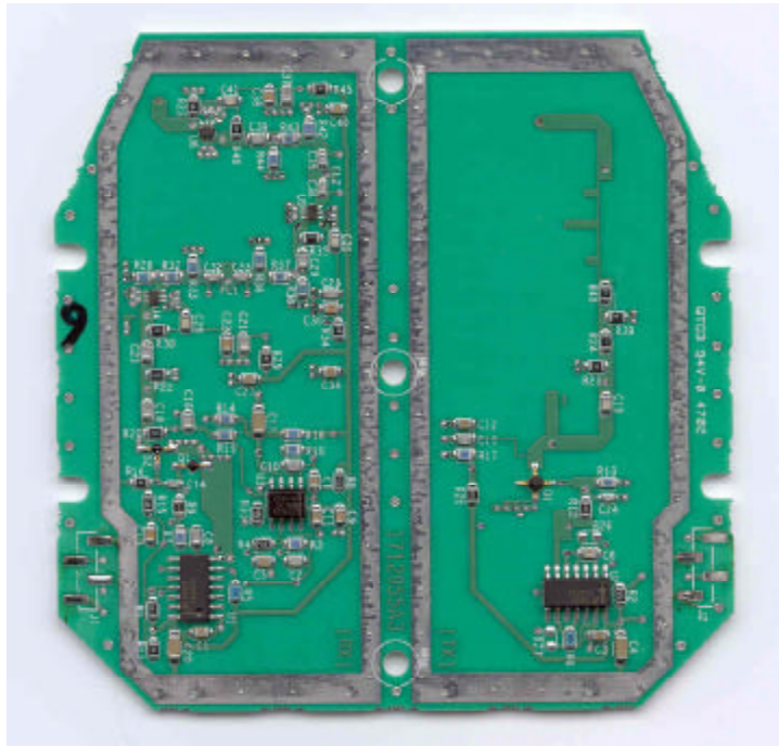
Antenna/RF PCB - Component Side
