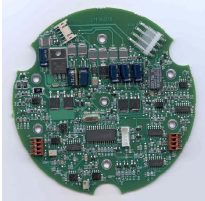
Processor PCB – Component Side
