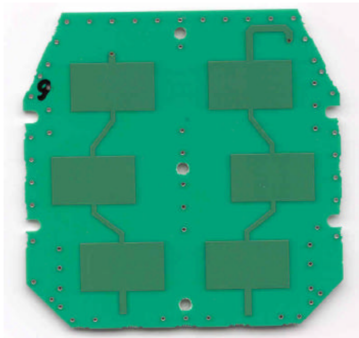
Antenna/RF PCB - Solder Side
