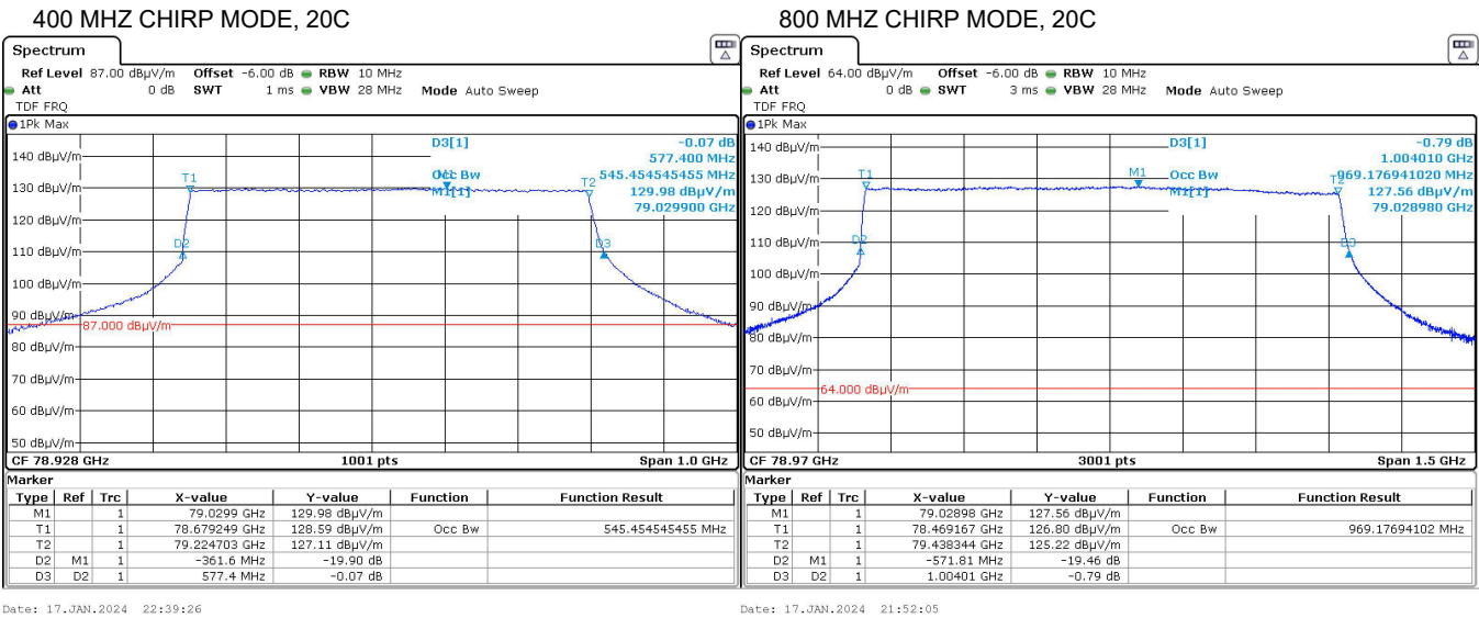
Figure 4.2.2 Example Intentional Emission Bandwidth.
