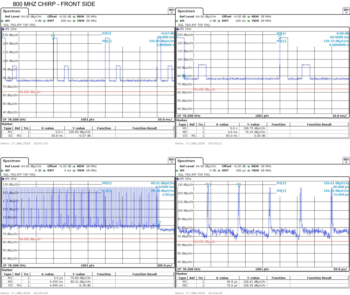
Figure 4.2.1 (ii) Example Pulsed Emission Characteristics (Duty Cycle).
