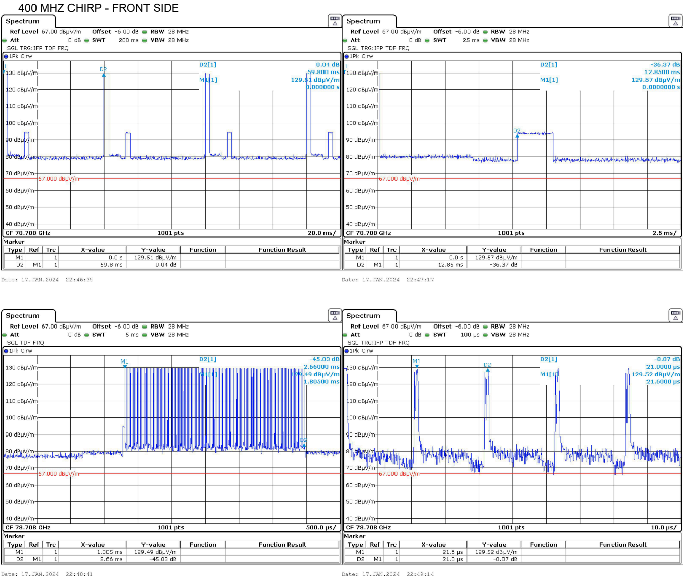
Figure 4.2.1 (i) Example Pulsed Emission Characteristics (Duty Cycle).
