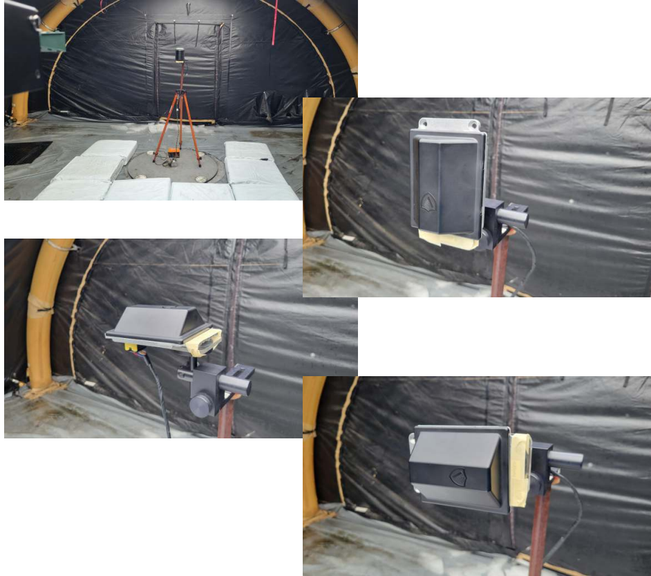
Figure 4.1.1 Radiated Emissions Test Setup Photograph(s).
