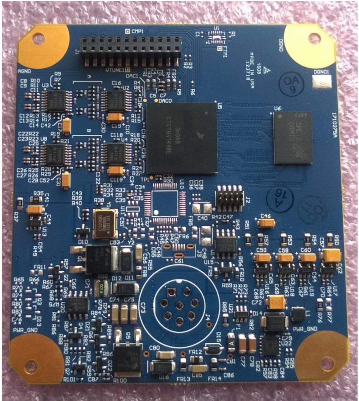
Processor PCA Front
