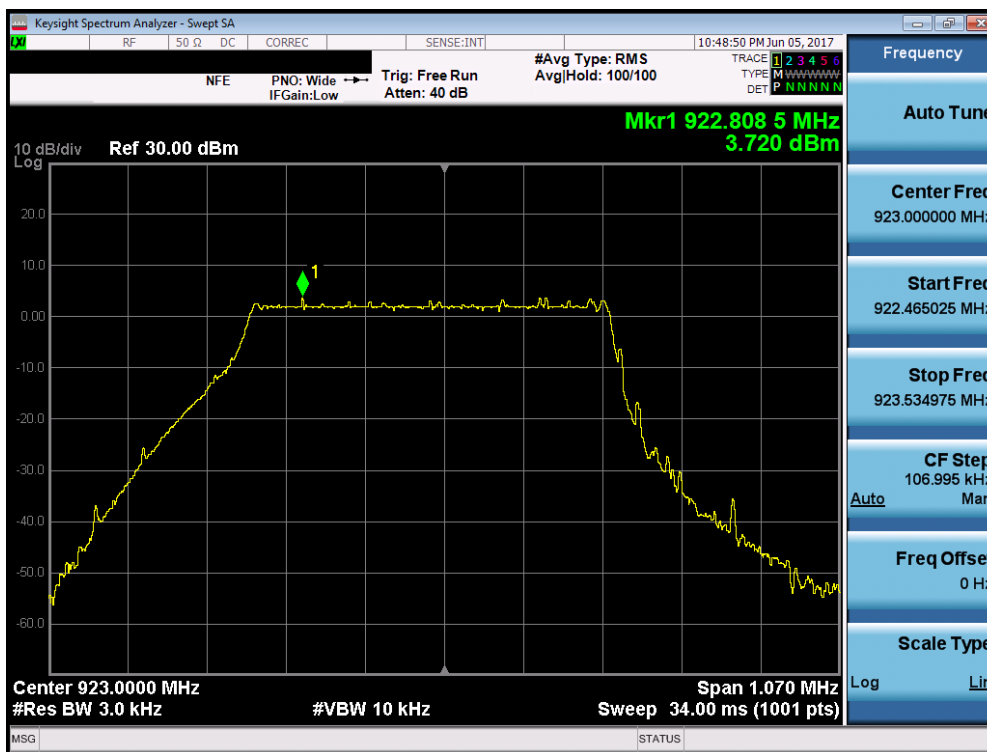
Plot 7-9. Power Spectral Density Plot (High Channel)
