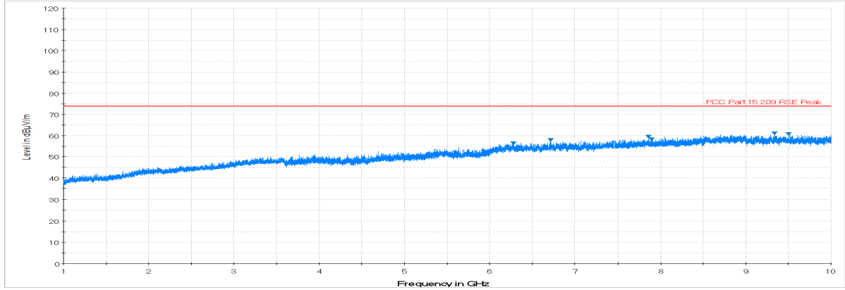
Plot 7-21. Radiated Spurious Plot above 1GHz (Mid Channel, Ant. Pol. V)
