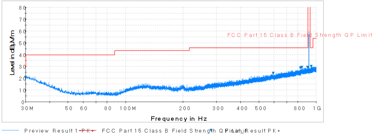
Plot 7-24. Radiated Spurious Plot below 1GHz (Pol. H)
