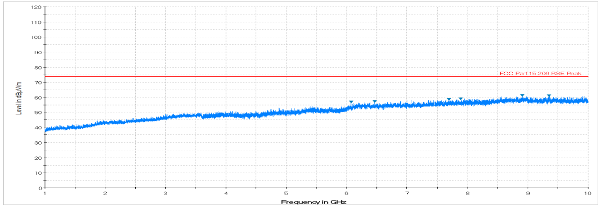
Plot 7-23. Radiated Spurious Plot above 1GHz (High Channel, Ant. Pol. V)
