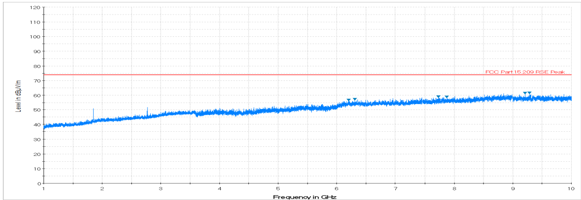
Plot 7-22. Radiated Spurious Plot above 1GHz (High Channel, Ant. Pol. H)
