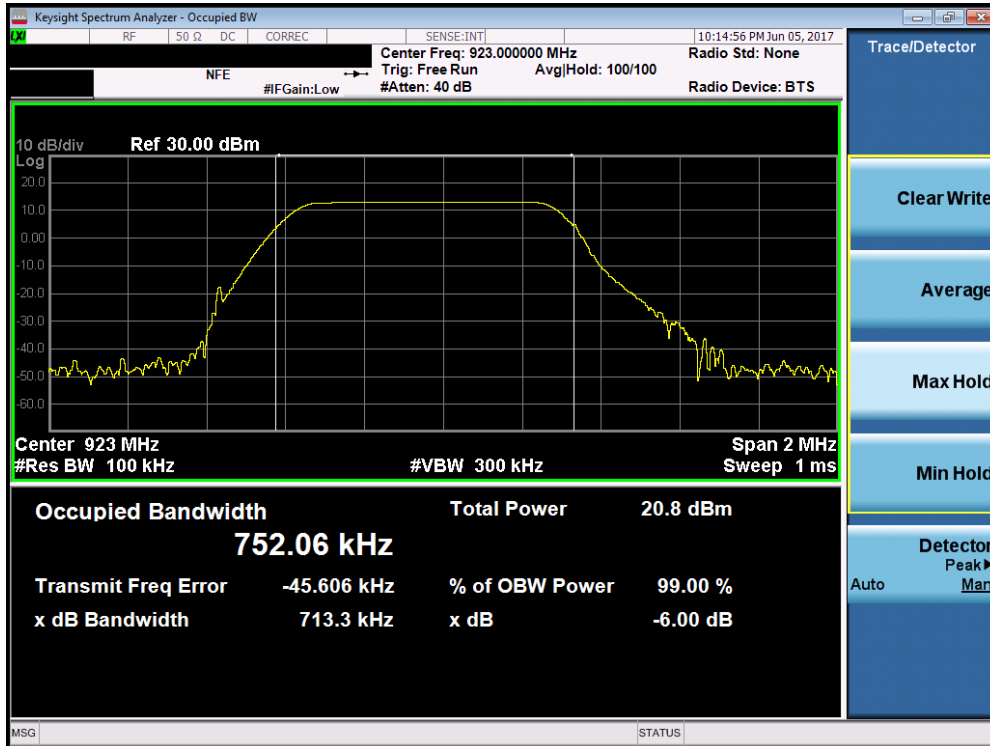
Plot 7-3. 6dB Bandwidth Plot (High Channel)
