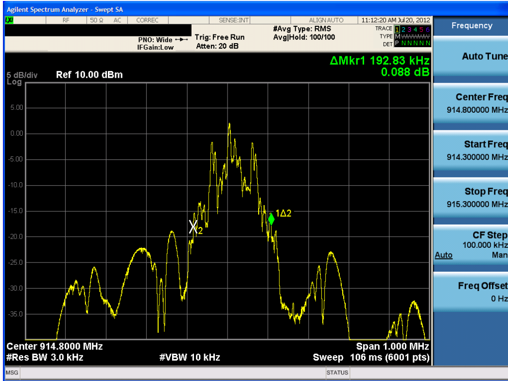
Plot 6-2. 20dB Bandwidth Plot (Mid Channel)
