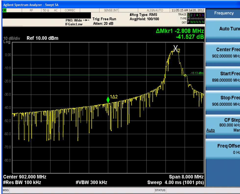
Plot 6-4. Lower Band Edge Plot (Hopping Disabled)
