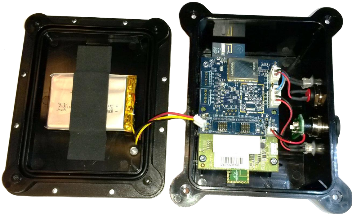
Internal Housing – Cover Removed:
