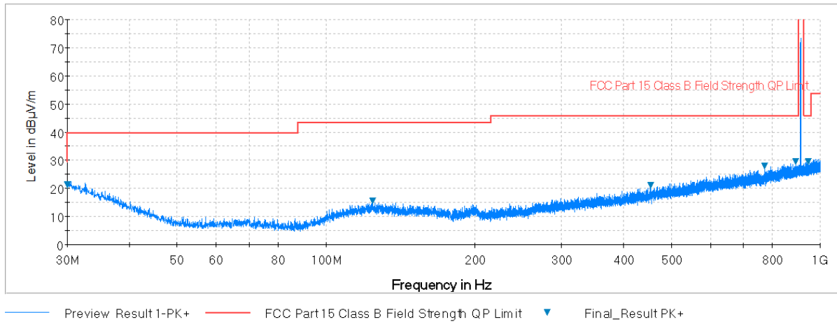
Plot 7-25. Radiated Spurious Plot below 1GHz (Pol. V)
