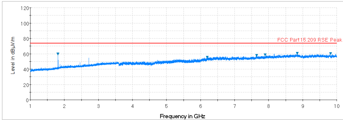
Plot 7-19. Radiated Spurious Plot above 1GHz (Low Channel, Ant. Pol. V)
