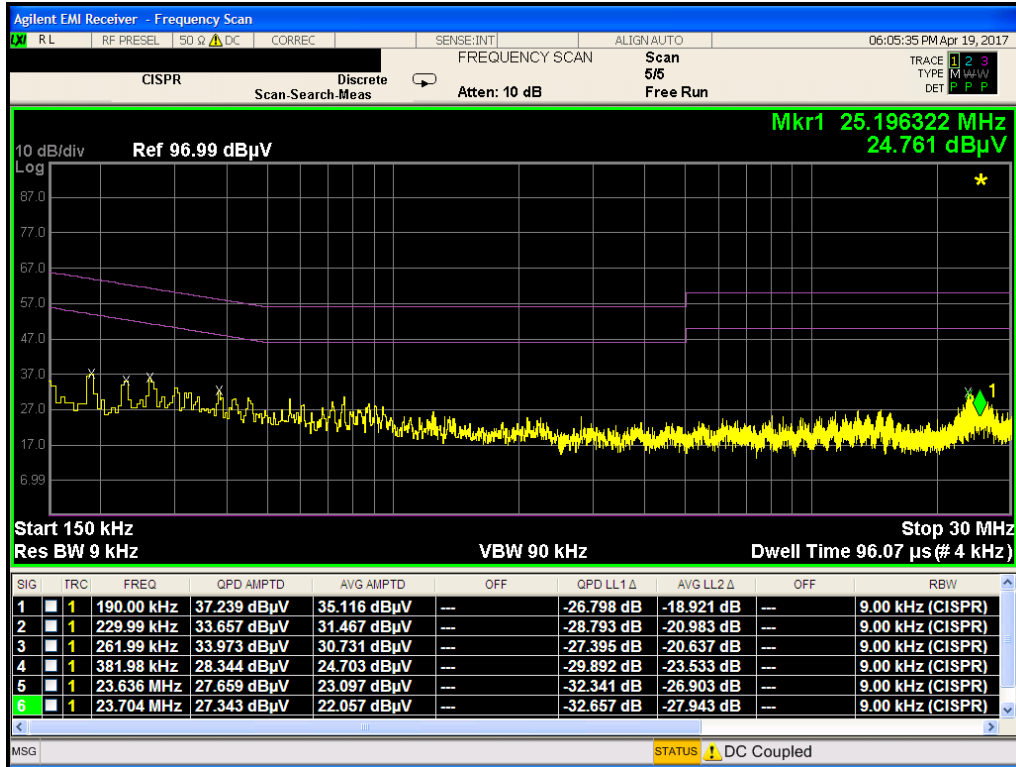
Plot 7-26. Line Conducted Plot with 802.11b (L1)
