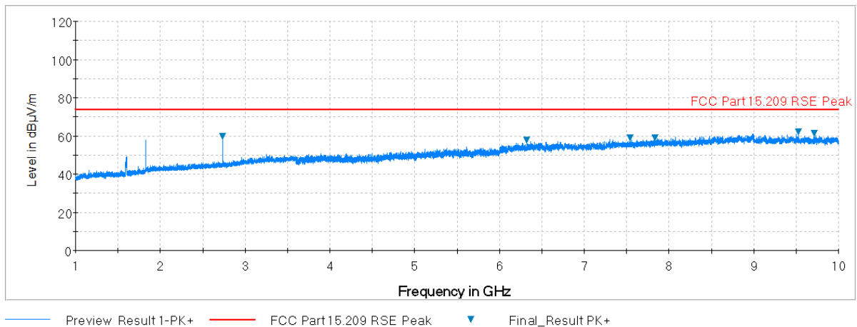
Plot 7-23. Radiated Spurious Plot above 1GHz (High Channel, Ant. Pol. V)
