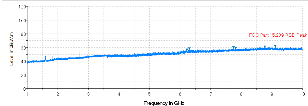
Plot 7-18. Radiated Spurious Plot above 1GHz (Low Channel, Ant. Pol. H)
