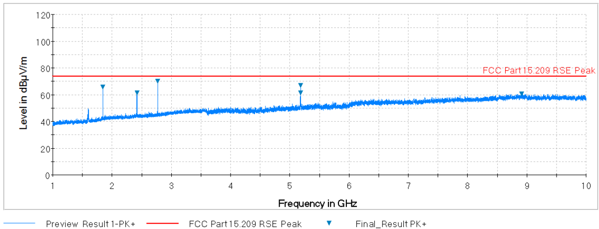
Plot 7-22. Radiated Spurious Plot above 1GHz (High Channel, Ant. Pol. H)
