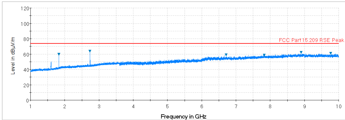
Plot 7-20. Radiated Spurious Plot above 1GHz (Mid Channel, Ant. Pol. H)
