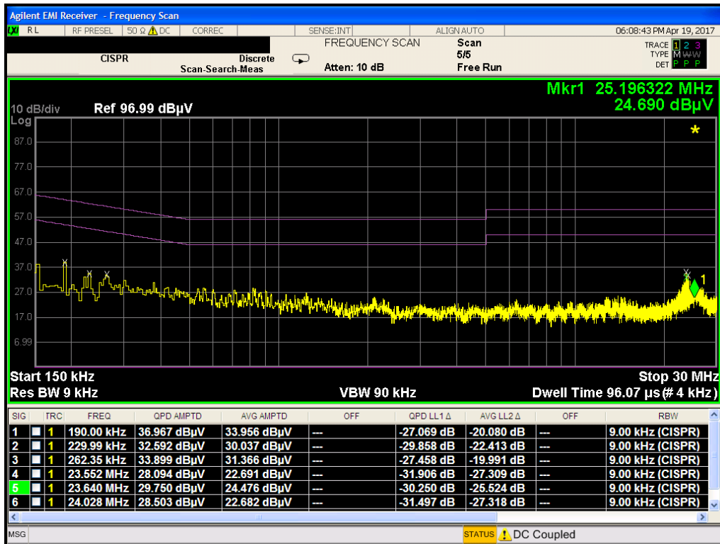
Plot 7-27. Line Conducted Plot with 802.11b (N)
