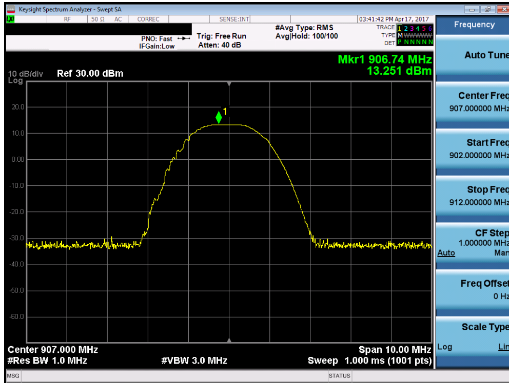
Plot 7-4. Conducted Output Power Measurements (Low Channel)
