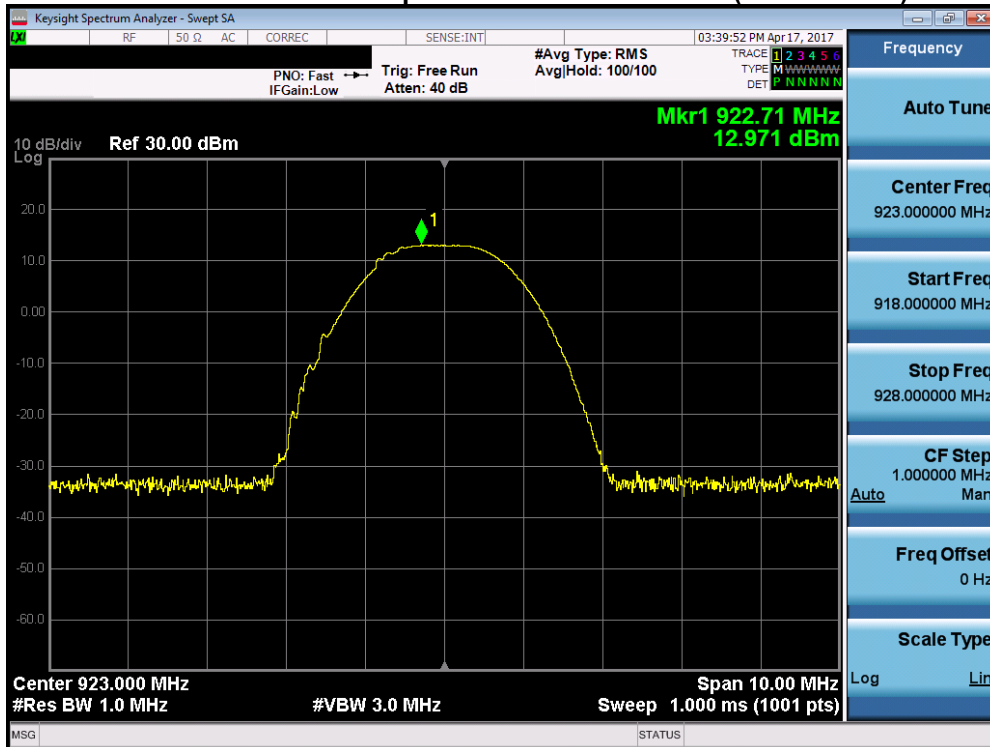
Plot 7-6. Conducted Output Power Measurements (High Channel)
