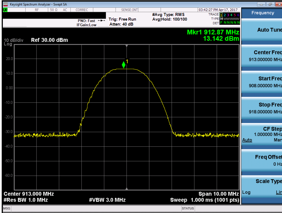
Plot 7-5. Conducted Output Power Measurements (Mid Channel)
