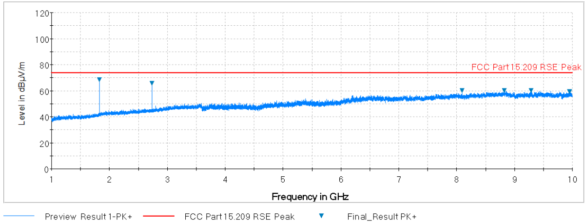
Plot 7-21. Radiated Spurious Plot above 1GHz (Mid Channel, Ant. Pol. V)
