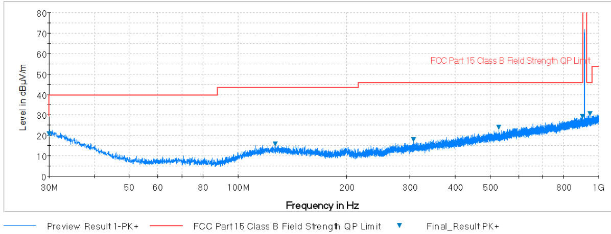
Plot 7-24. Radiated Spurious Plot below 1GHz (Pol. H)
