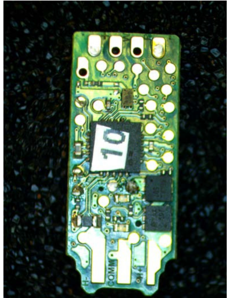
PCB photo bottom side A1006017RBT Rev 4.01
