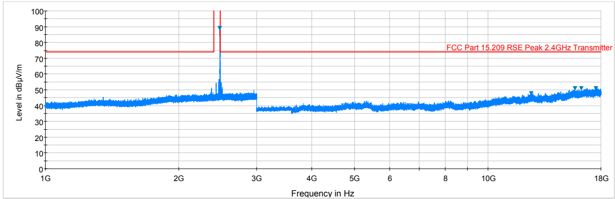
Plot 6-7. Radiated Spurious Plot above 1GHz (BTLE – Ch. 19, Ant. Pol. V)
