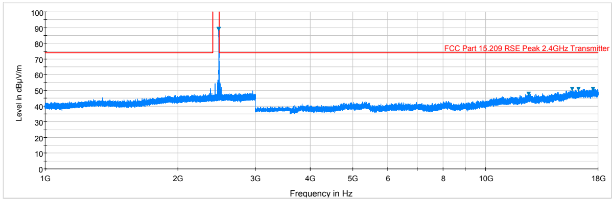
Plot 6-9. Radiated Spurious Plot above 1GHz (BTLE – Ch. 39, Ant. Pol. V)
