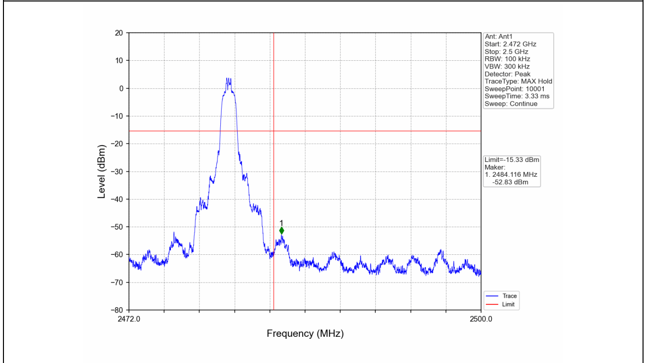
Pi/4DQPSK_2DH5_HCH_2480MHz_Ant1_NTNV
