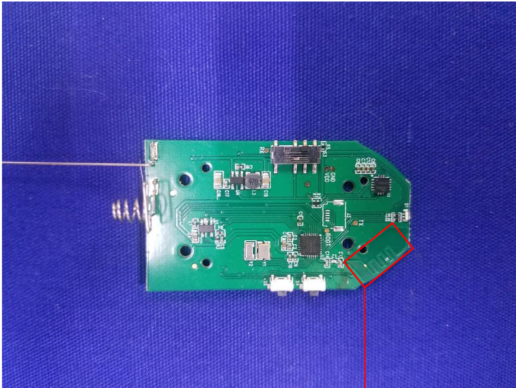
BT& 2.4G SRD Antenna
