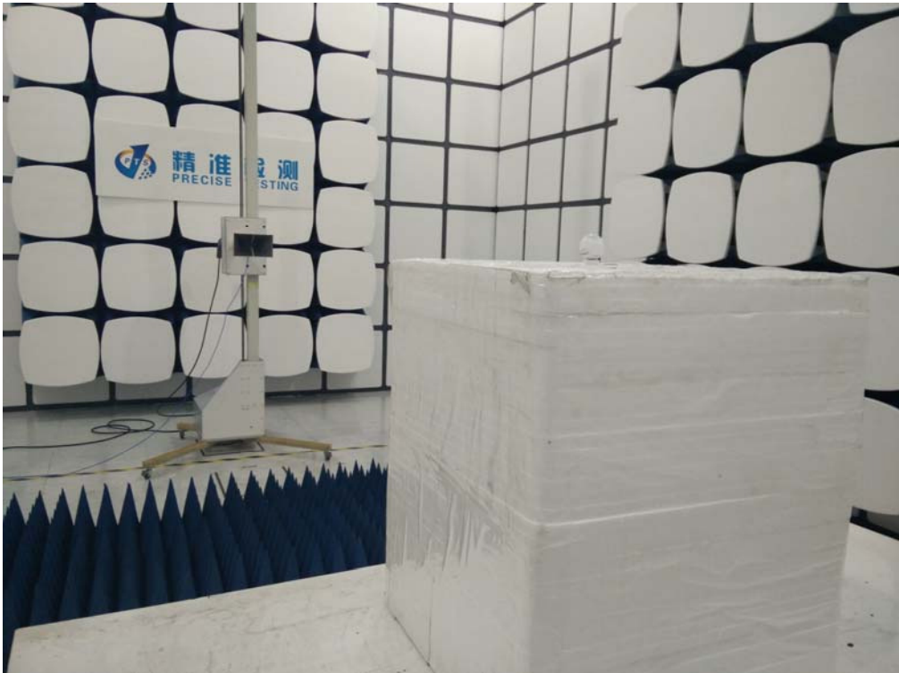
Above 1GHz
