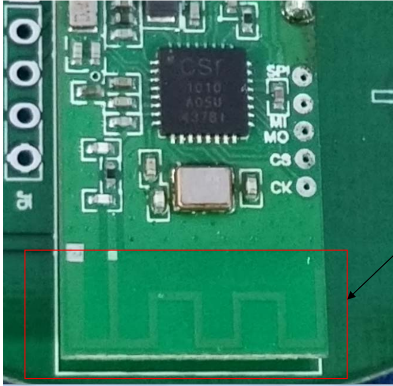
Bluetooth Antenna
