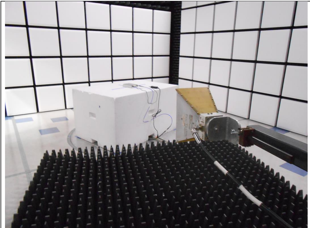
RF Radiated #4
