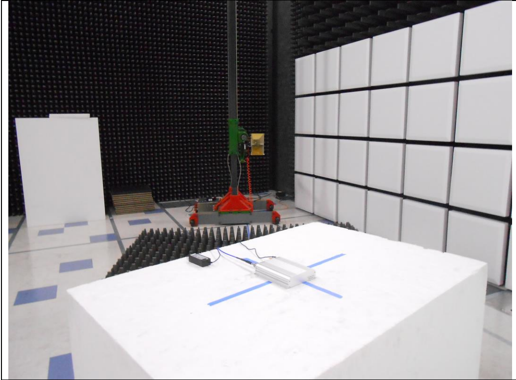
RF Radiated #4
