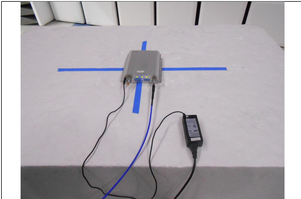
RF Radiated #2
