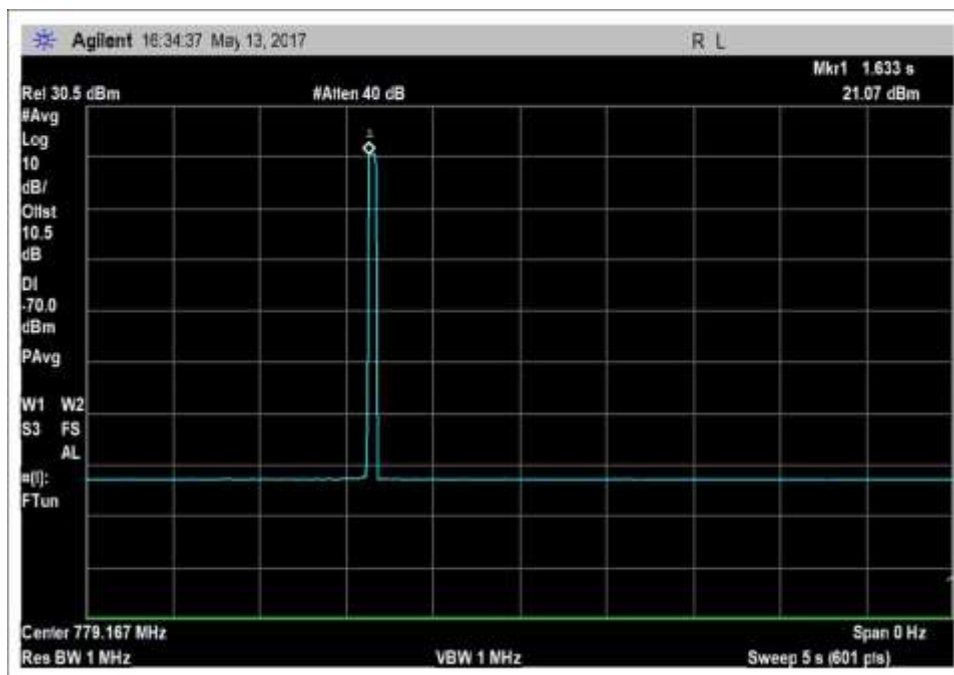
UL-776-787MHz Peak
