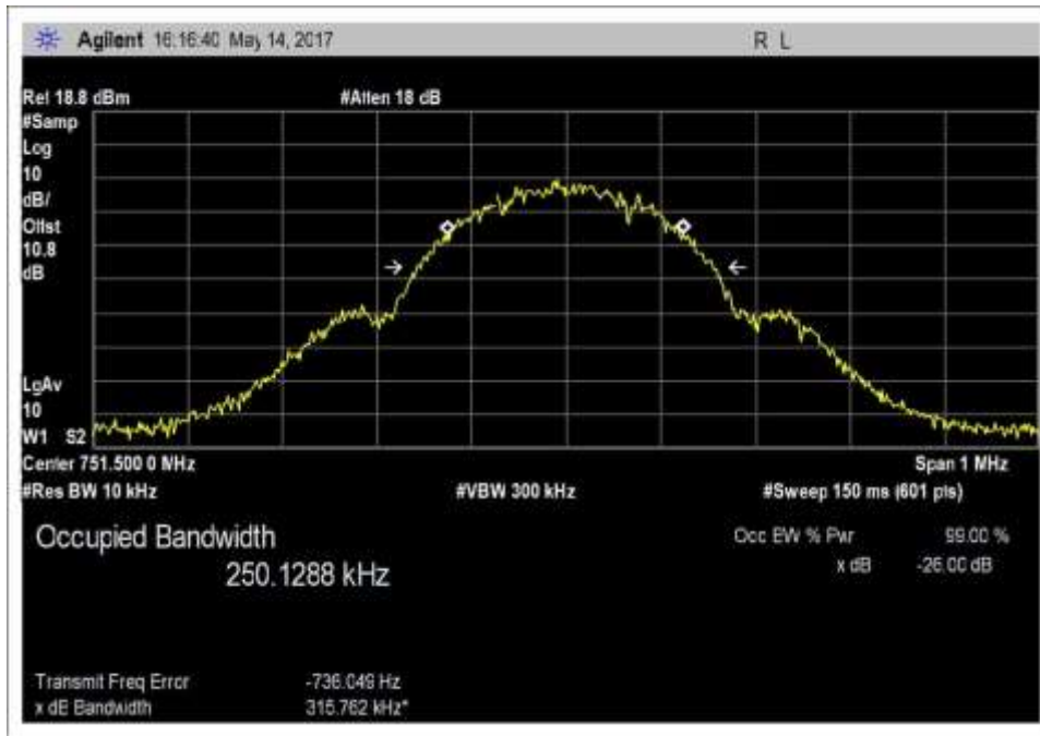
Output_OBW_DL_746-757MHz_GSM
