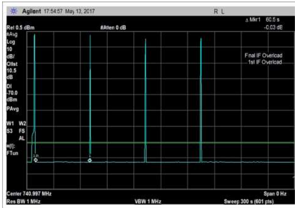
DL- 728-746MHz_300s
