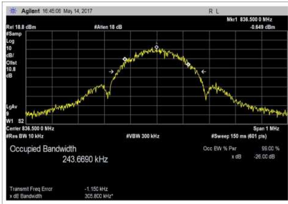
Output_OBW_UL_824-849MHz_EDGE
