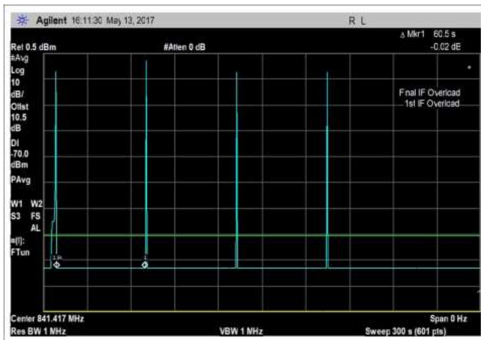
UL-824-849MHz_300s
