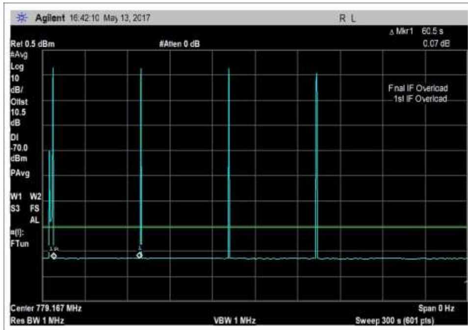
UL-776-787MHz_300s
