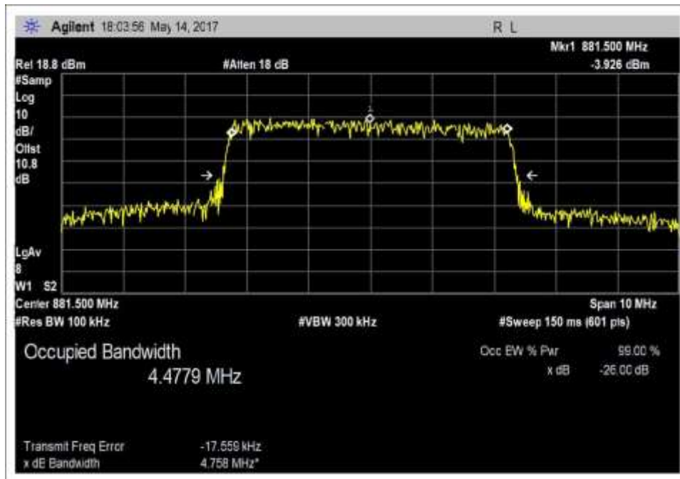
Output_OBW_DL_869-894MHz_LTE
