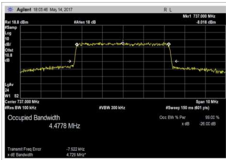
Output_OBW_DL_728-746MHz_LTE
