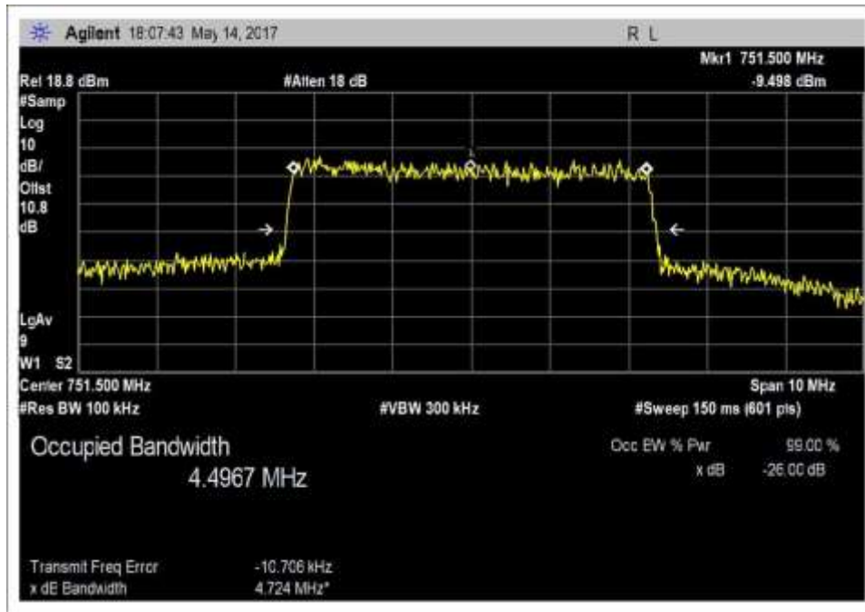
Output_OBW_DL_746-757MHz_LTE
