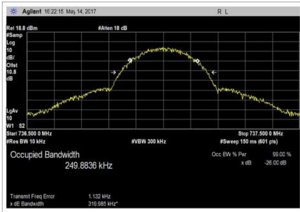
Output__OBW_DL_728-746MHz_EDGE
