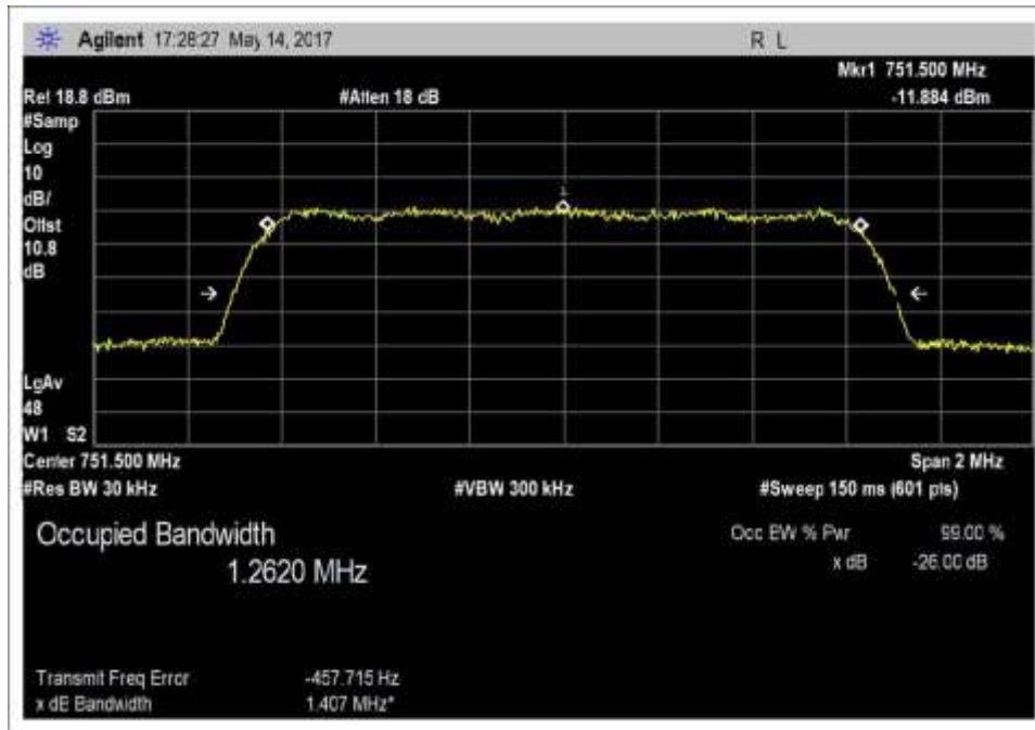
Output_OBW_DL_746-757MHz_CDMA
