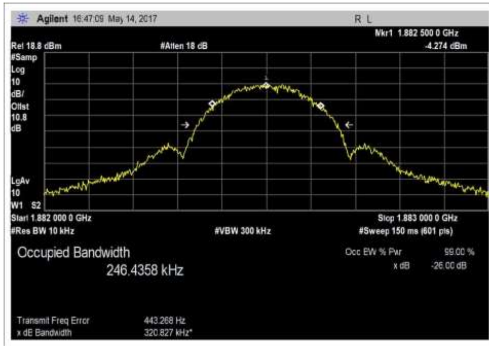
Output_OBW_UL_1850-1915MHz_EDGE
