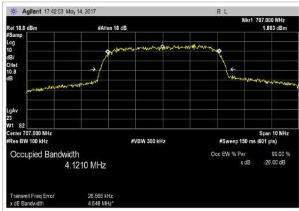
Output_OBW_UL_698-716MHz_WCDMA
