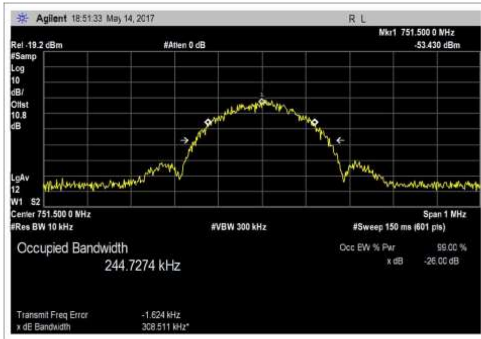
Input_OBW_DL_746-757MHz_EDGE
