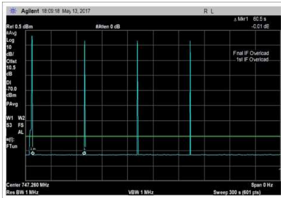
DL- 746-757MHz_300s
