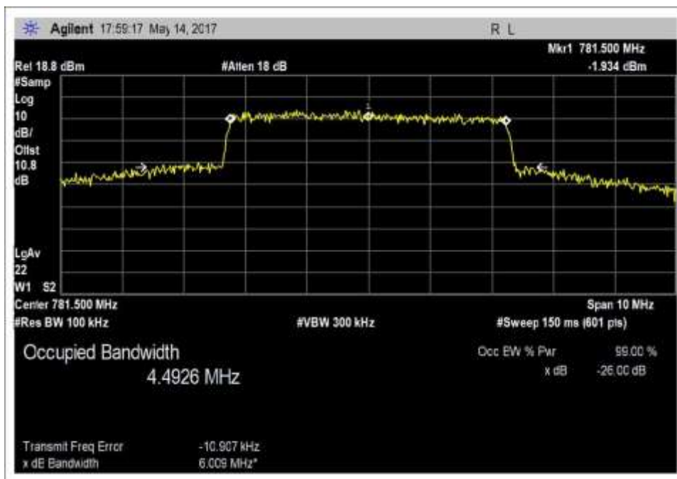
Output_OBW_UL_776-787MHz_LTE
