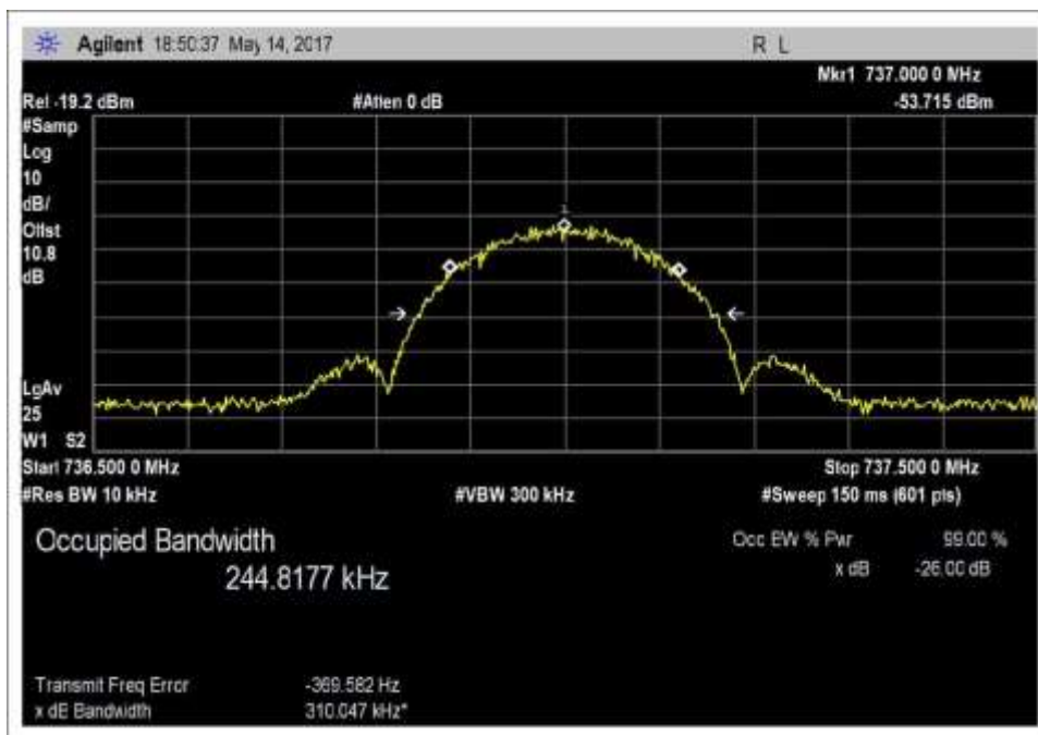
Input_OBW_DL_728-746MHz_EDGE
