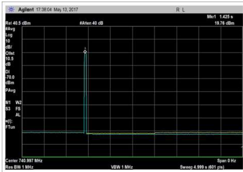
DL- 728-746MHz_Peak
