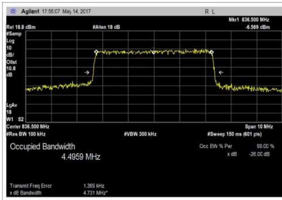
Output_OBW_UL_824-849MHz_LTE
