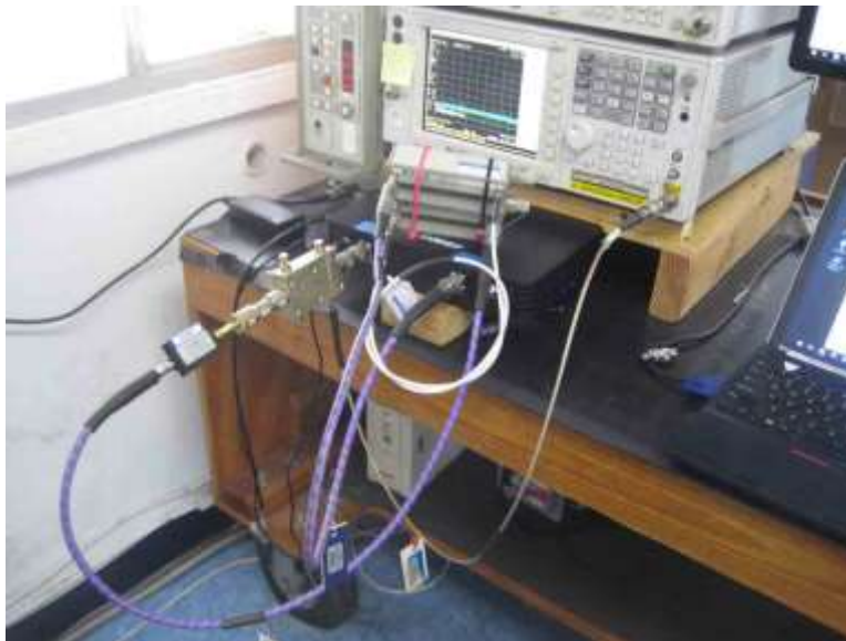
Section 7.11 Oscillation Timing Test Setup
