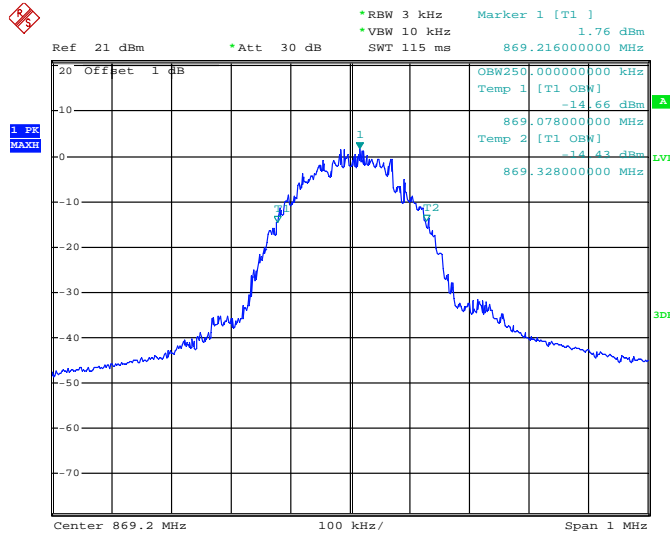
Output(Low channel)
