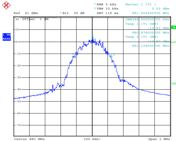
Output(Middle channel)
