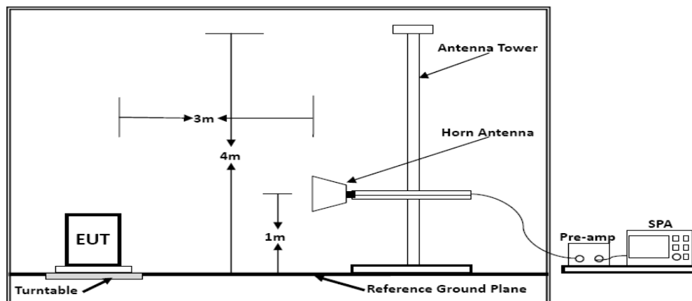
Above 1GHz
