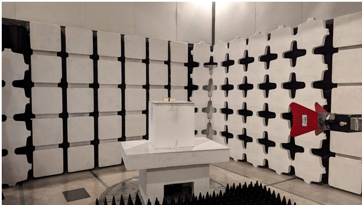
OWS-NIC511-LTE Spurious Emissions 1-18GHz
