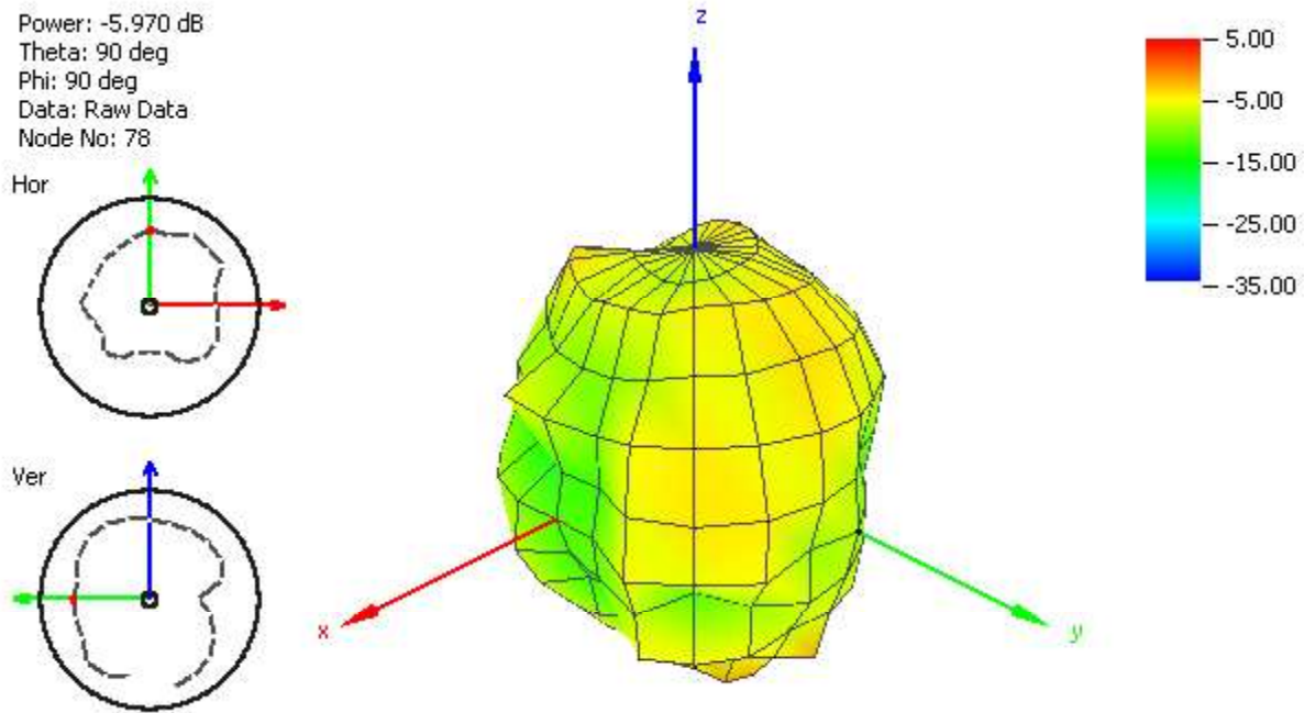
Figure 36. Radiation Pattern at 2400 MHz of G30 Antenna on 30x30cm metal plate.
