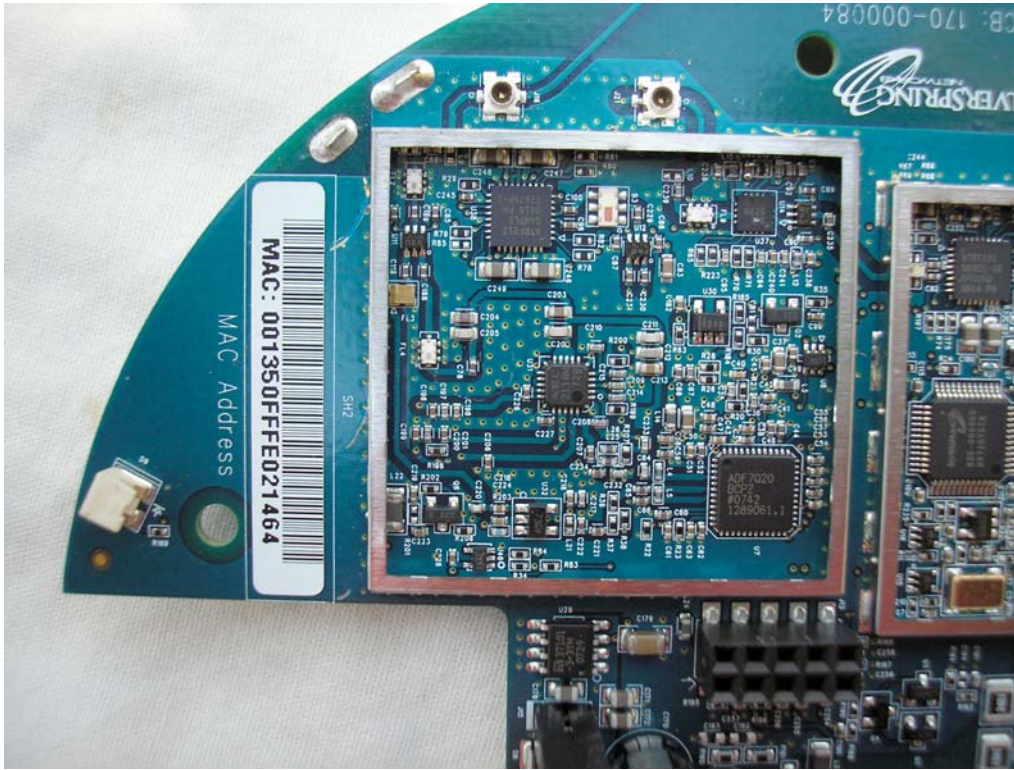
FHSS Radio
