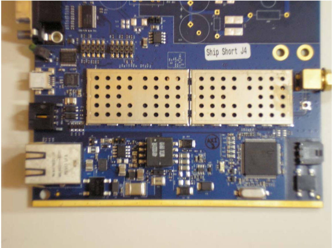
Detail power supply section
