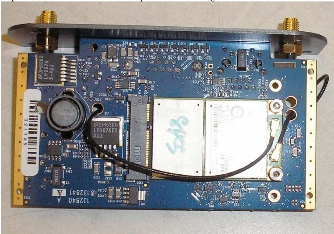
Top side of Sierra Wireless interface pcb inside mounting box
