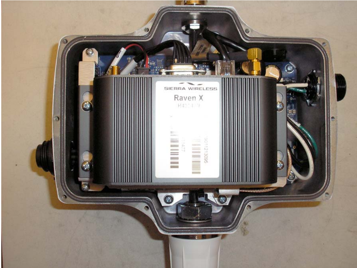
Cover off, showing Sierraa Wireless RF module board metal mounting box cover
