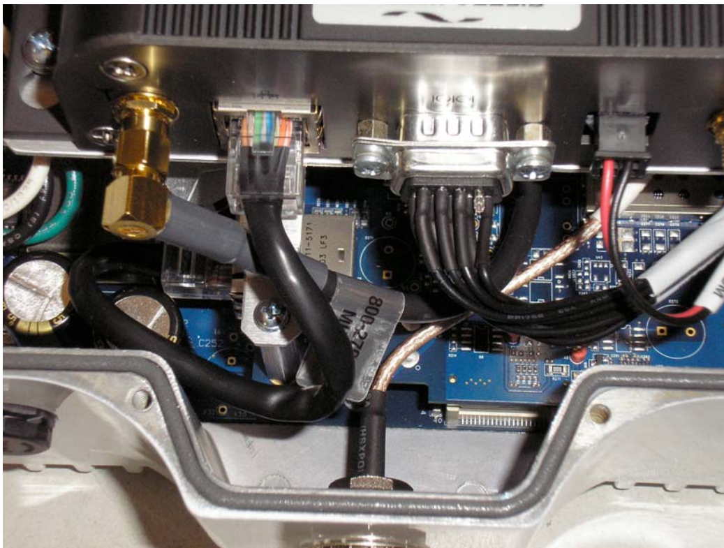
Detail of control, antenna, power and Ethernet connections on mounting box
