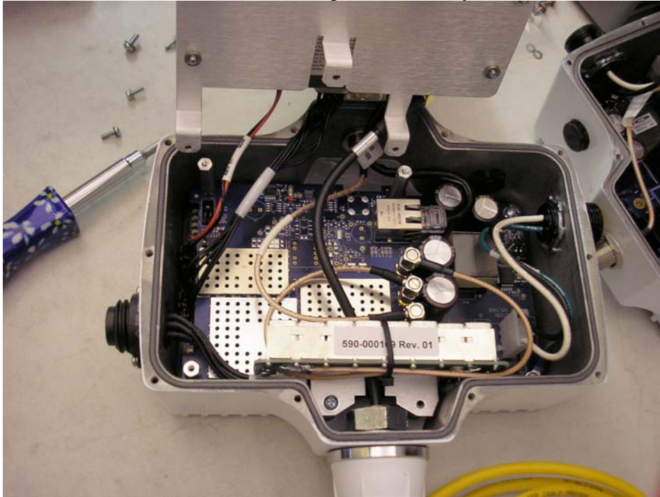
The Sierra Wireless power, control and Ethernet connections are made to existing sockets on the original NIC505 board. No new connectors were required to be put on the board.
