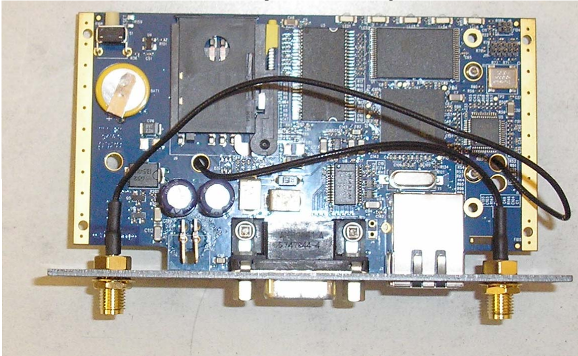
Bottom side of Sierra Wireless interface pcb inside mounting box
