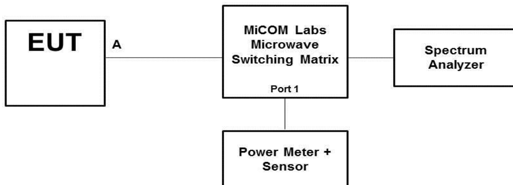
Conducted Test Measurement Setup
