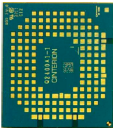
PHS8-P Bottom Side
