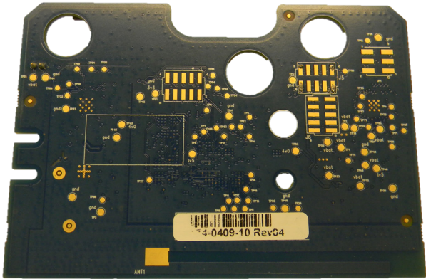
PCB Bottom Side (no potting)
