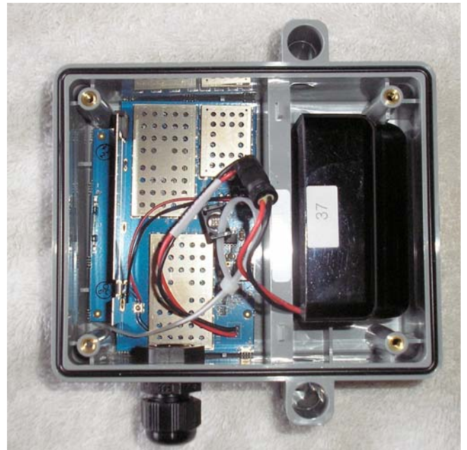
Radio module in plastic box with battery installed
