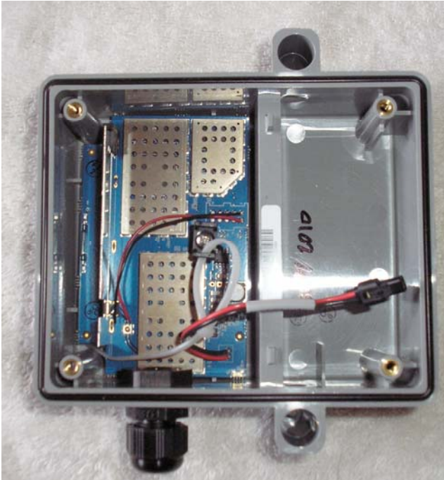
Radio module in plastic box housing
