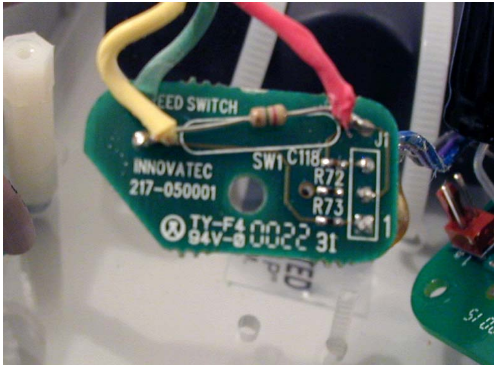
Figure 7 Component Side View of Reed Switch Board
