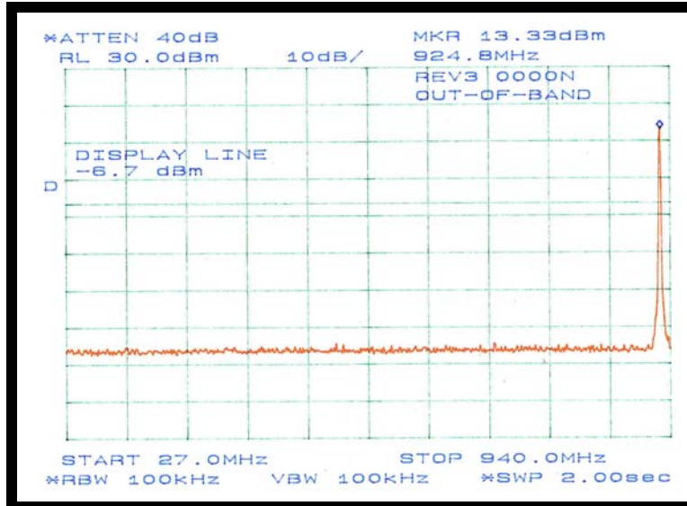
Figure 27: Plot of 100 kHz Bandwidth Out-of-Band Measurement at Channel 11
