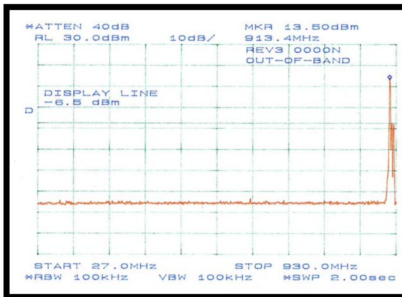
Figure 24: Plot of 100 kHz Bandwidth Out-of-Band Measurement at Channel 6
