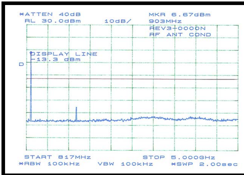
Figure 22: Plot of 100 kHz Bandwidth Out-of-Band Measurement at CH 0
