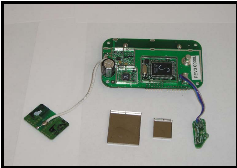
Figure 41: Component with Shield off
