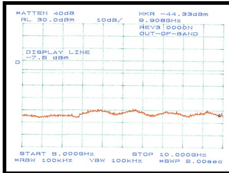
Figure 26: Plot of 100 kHz Bandwidth Out-of-Band Measurement at Channel 6
