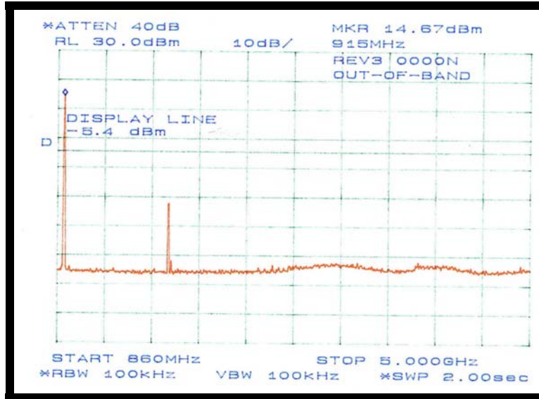
Figure 25: Plot of 100 kHz Bandwidth Out-of-Band Measurement at Channel 6
