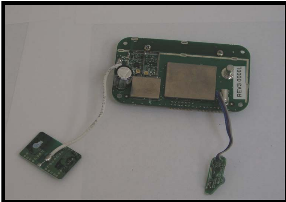
Figure 40: Component Solder View
