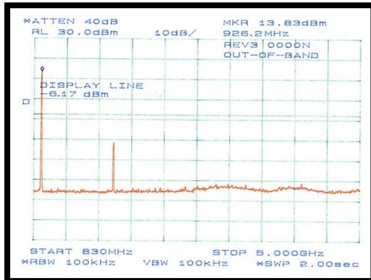
Figure 28: Plot of 100 kHz Bandwidth Out-of-Band Measurement at Channel 11
