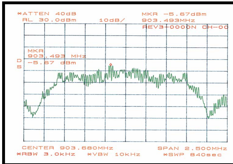
Figure 12: Plot of Spectral Density Measurement at Channel 0
