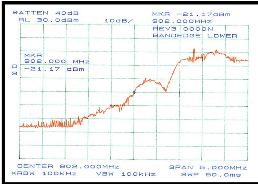
Figure 18: Plot of Lower Band-Edge Measurement at 902MHz
