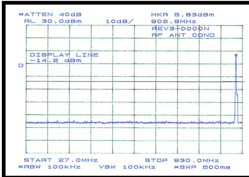
Figure 21: Plot of 100 kHz Bandwidth Out-of-Band Measurement at CH 0
