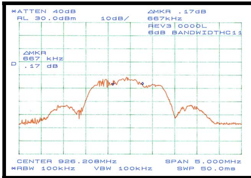
Figure 17: Plot of 6dB Bandwidth Measurement at Channel 11
