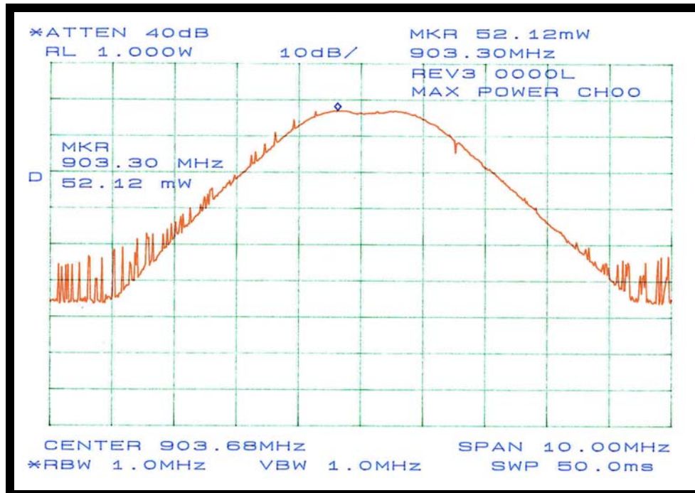
Figure 9: Plot of Maximum Power Measurement at Channel 0
