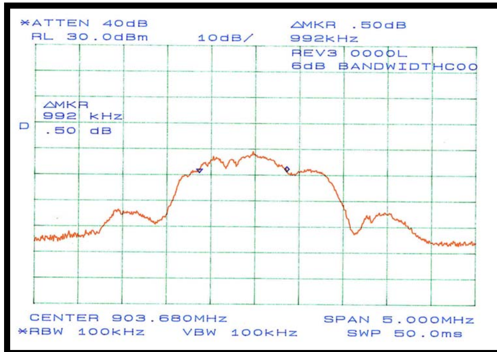
Figure 15: Plot of 6dB Bandwidth Measurement at Channel 0
