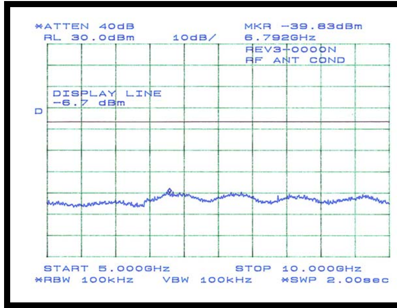
Figure 29: Plot of 100 kHz Bandwidth Out-of-Band Measurement at Channel 11
