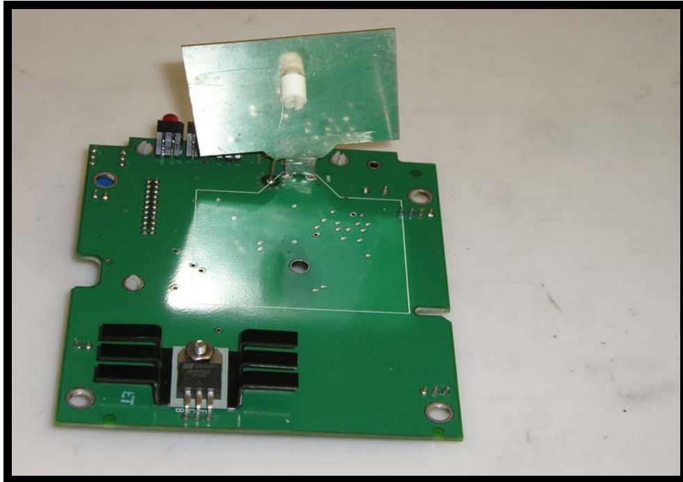
Figure 5: Solder View with Shield off
