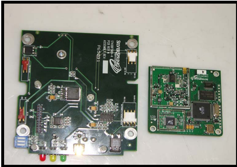
Figure 3: Component View With Shield Off
