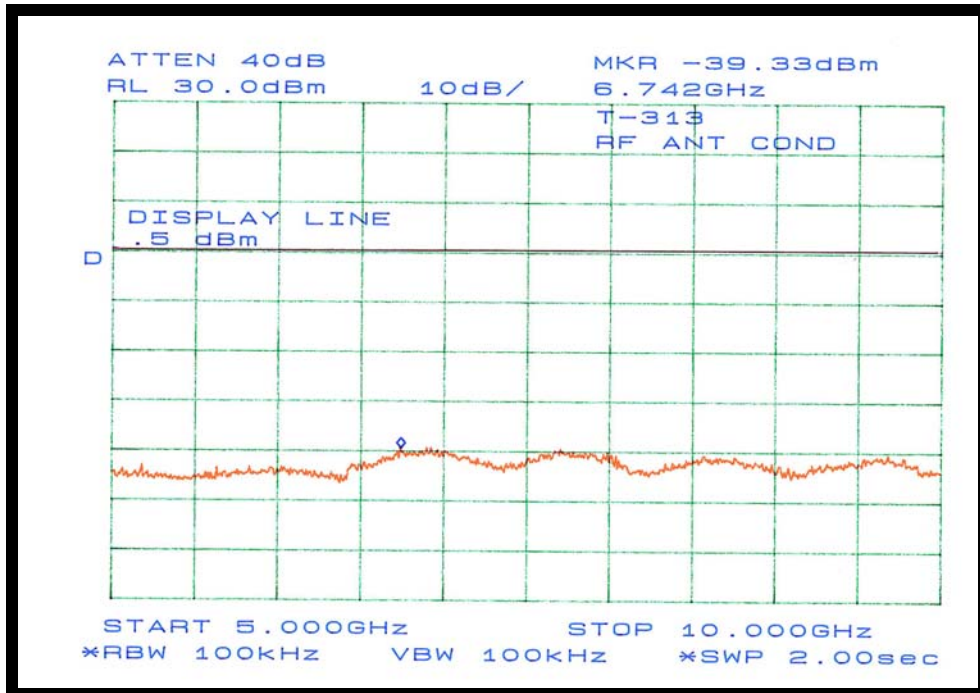
Figure 28: Plot of 100 kHz Bandwidth Out-of-Band Measurement at Ch 6 (5 to 10 GHz)
