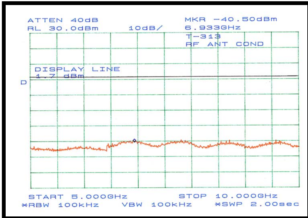
Figure 25: Plot of 100 kHz Bandwidth Out-of-Band Measurement at Ch 0 (5 GHz to 10 GHz)
