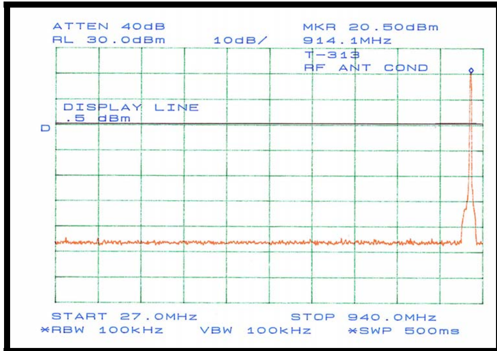
Figure 26: Plot of 100 kHz Bandwidth Out-of-Band Measurement at Ch 6 (27MHz to 940 MHz)
