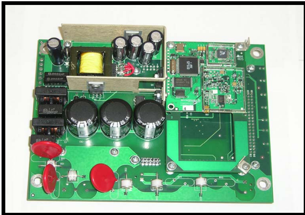
Figure 44: Component View with Shield off (View 1)
