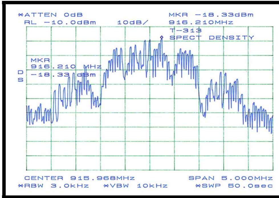
Figure 13: Plot of Spectral Density Measurement at Channel 6
