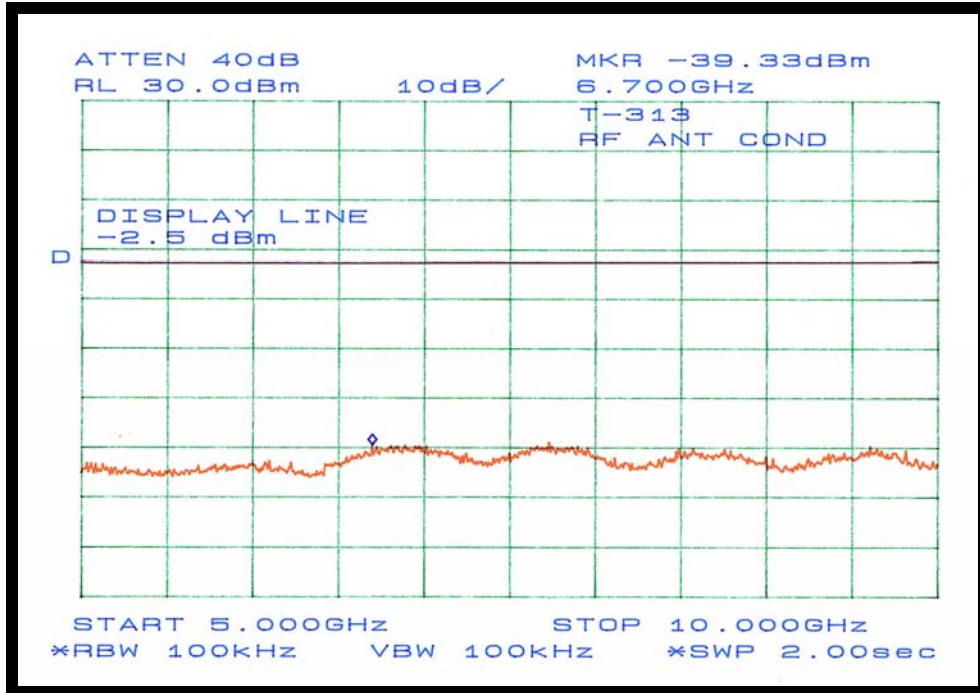
Figure 31: Plot of 100 kHz Bandwidth Out-of-Band Measurement at Ch 11(5 GHz – 10 GHz)
