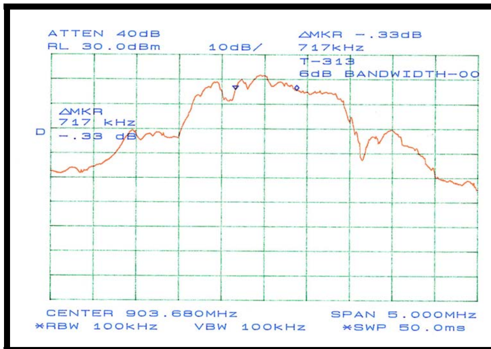
Figure 17: Plot of 6dB Bandwidth Measurement at Channel 0
