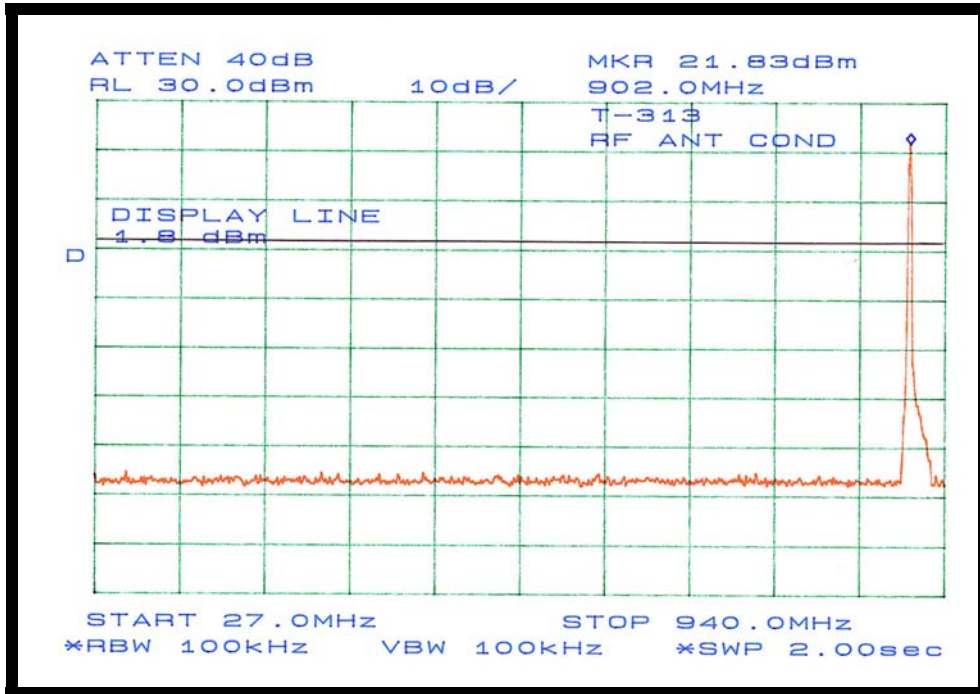
Figure 23: Plot of 100 kHz Bandwidth Out-of-Band Measurement at Ch 0 (27 MHz – 940 MHz)
