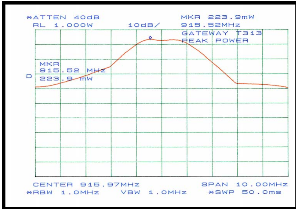
Figure 10: Plot of Maximum Power Measurement at Channel 6
