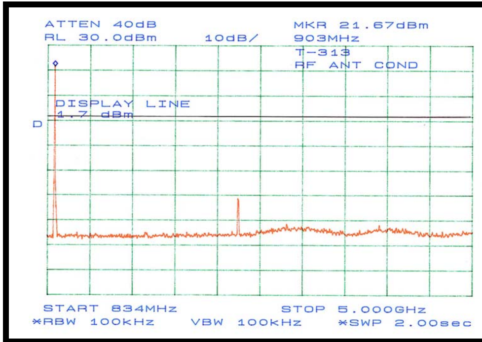
Figure 24: Plot of 100 kHz Bandwidth Out-of-Band Measurement at Ch 0 (834 MHz to 5 GHz))
