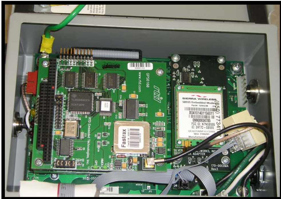
Figure 40: EUT Internal View1
