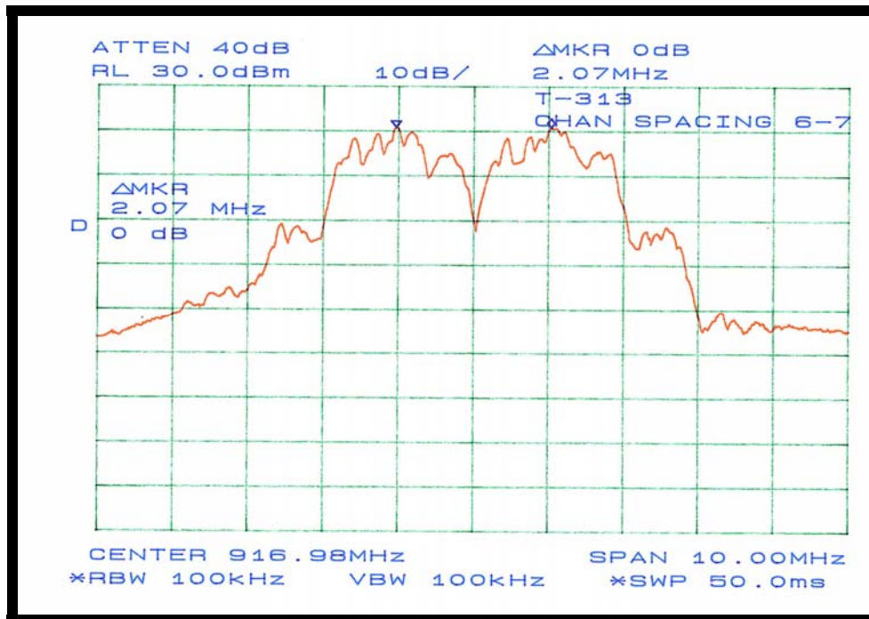
Figure 8: Plot of Channel Separation Measurement at 916.98 MHz
