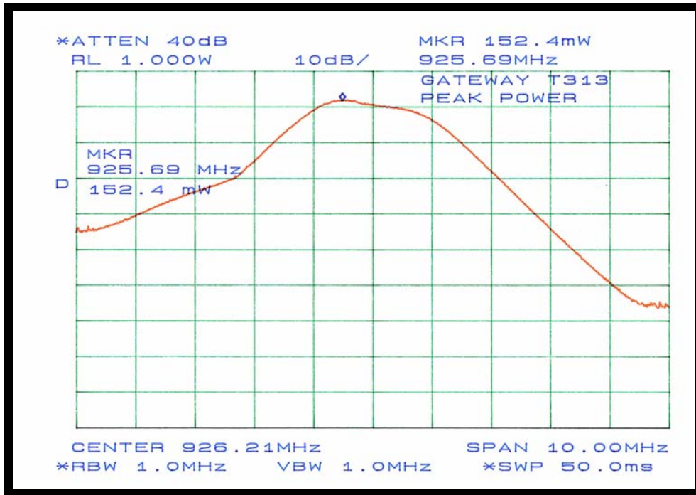
Figure 11: Plot of Maximum Power Measurement at Channel 11
