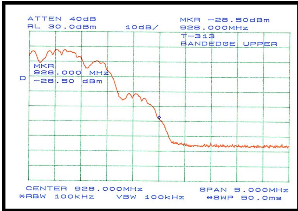
Figure 21: Plot of Band-Edge Measurement at 928MHz
