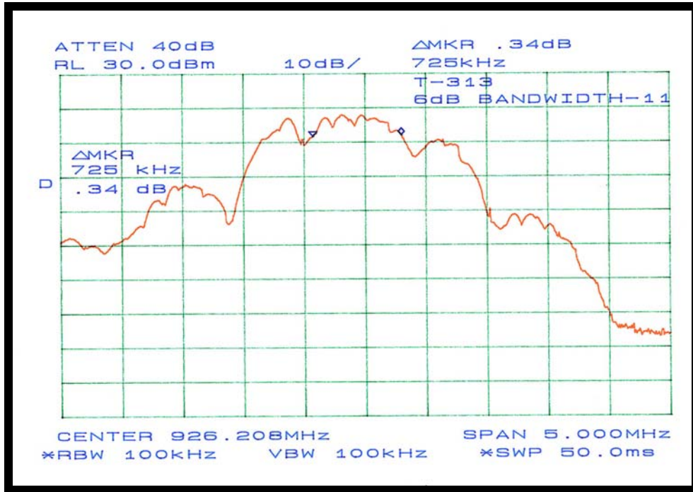
Figure 19: Plot of 6dB Bandwidth Measurement at Channel 11
