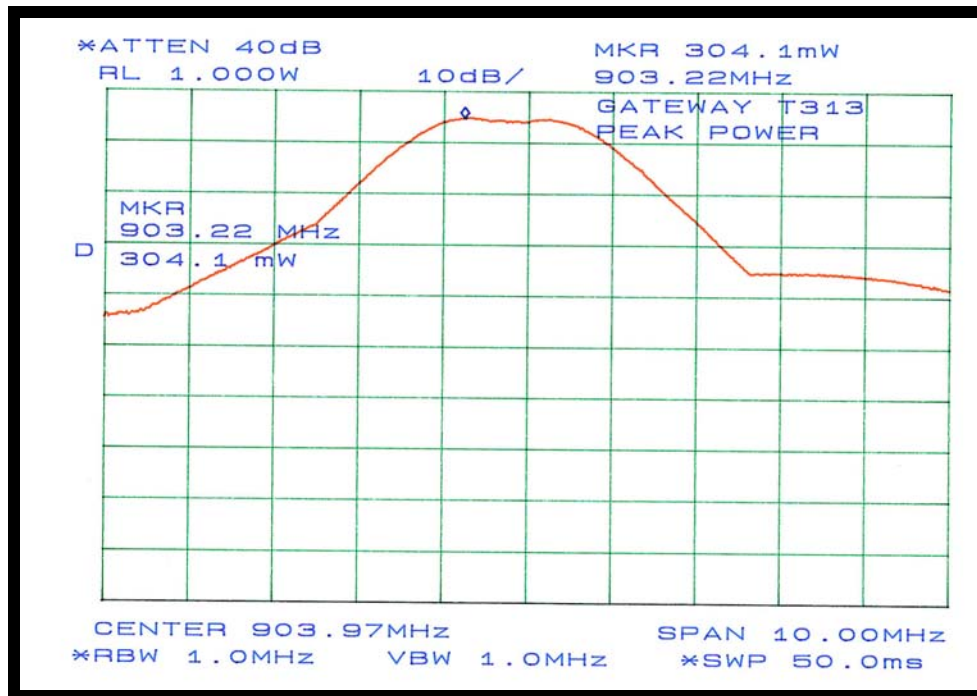
Figure 9: Plot of Maximum Power Measurement at Channel 0
