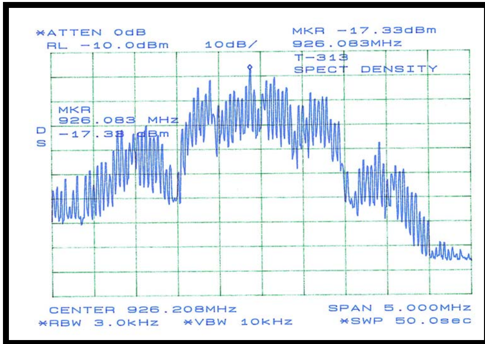
Figure 14: Plot of Spectral Density Measurement at Channel 11
