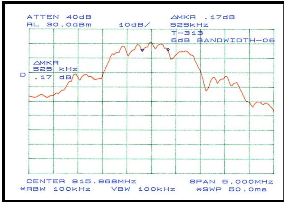
Figure 18: Plot of 6dB Bandwidth Measurement at Channel 6
