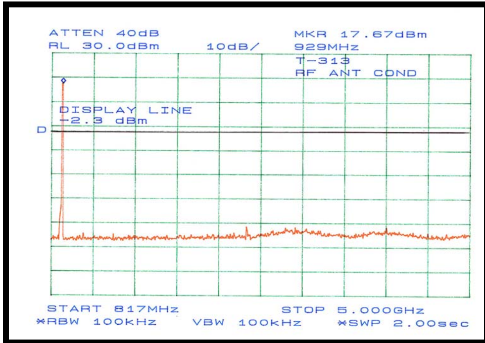
Figure 30: Plot of 100 kHz Bandwidth Out-of-Band Measurement at Ch 11(817 MHz to 5 GHz)
