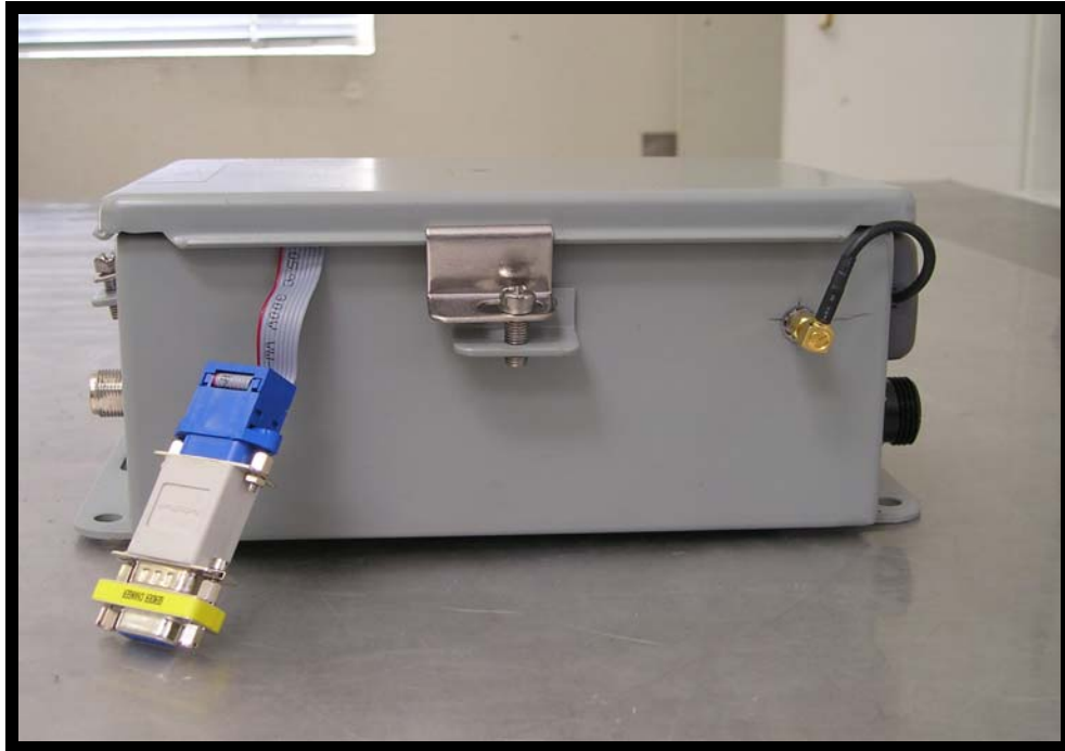
Figure 5: EUT Side View
