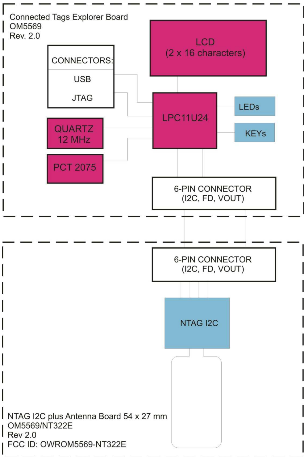
Picture 1: NTAG I 2 C plus Explorer Kit - Block Diagram
