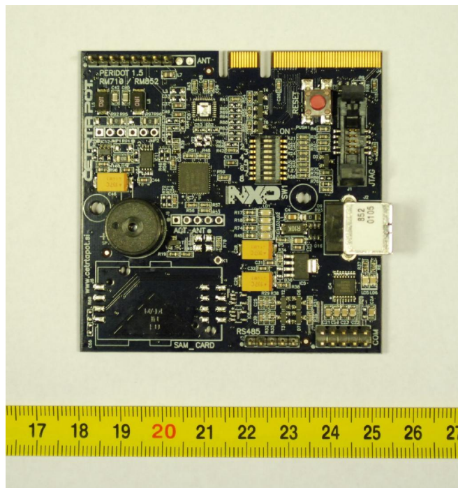
Picture 1: RD852 reader pcb - top side
