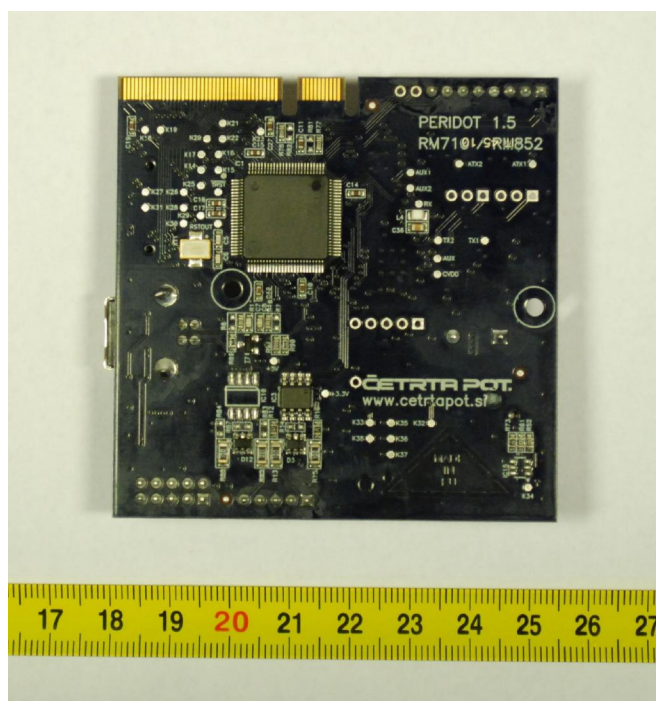
Picture 2: RD852 reader pcb - bottom side
