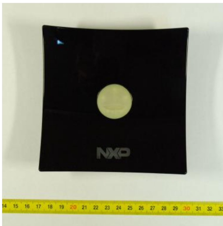
Picture 4: RD710 reader - top side
